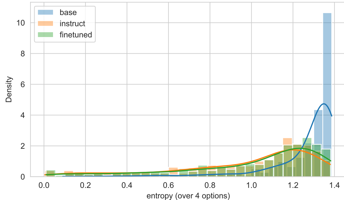
Entropy distribution: SimpleMC
