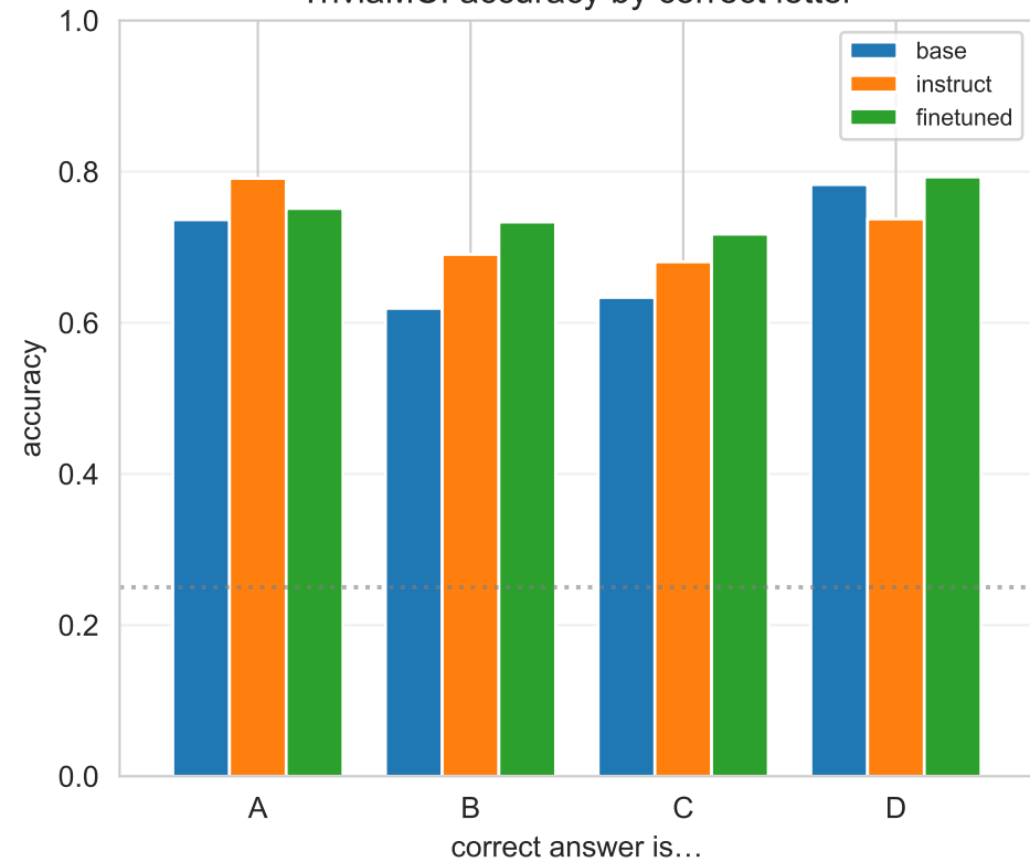
TriviaMC: accuracy by correct letter
