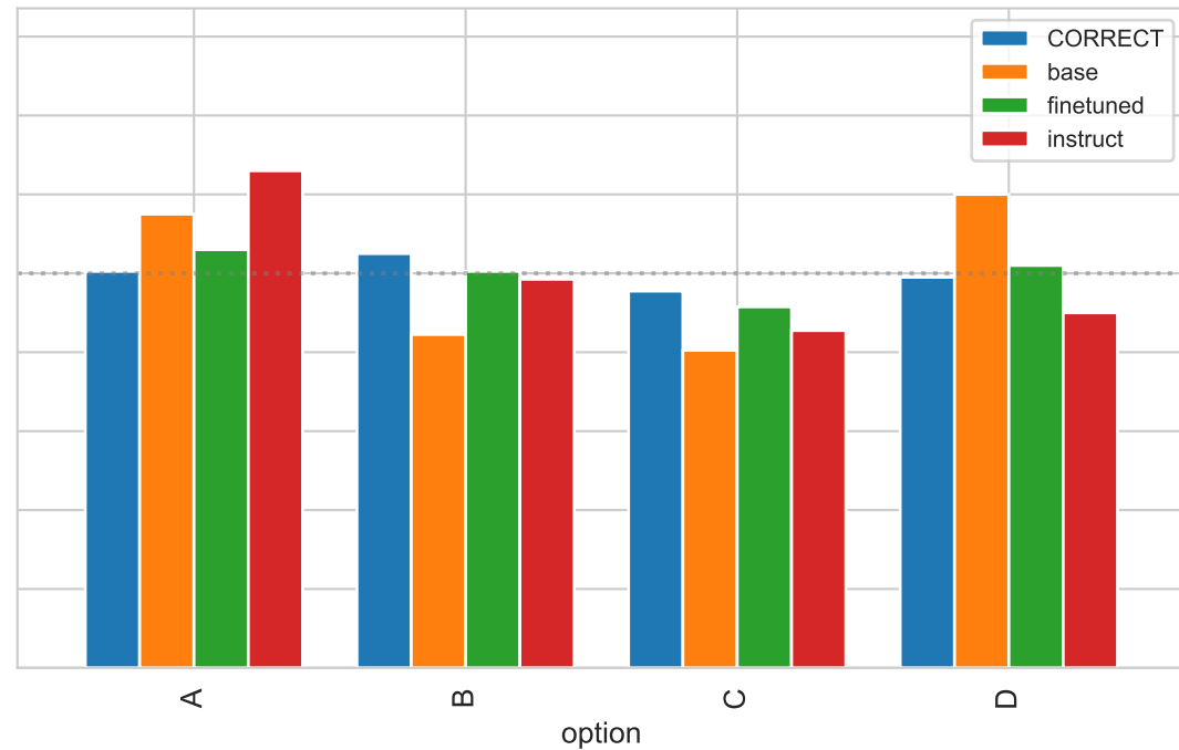
MC chosen answer — TriviaMC
