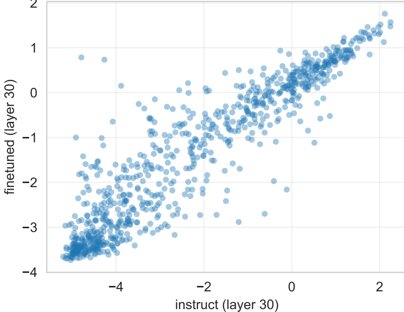
TriviaMC: instruct vs finetuned Spearman \rho = 0.920 ( p=0.00e+00 )
