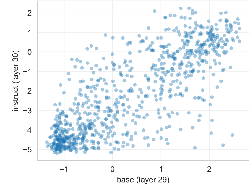
TriviaMC: base vs instruct Spearman \rho = 0.784 ( p=1.16e-167 )
