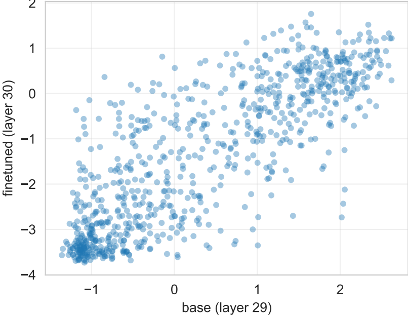
TriviaMC: base vs finetuned Spearman \rho = 0.811 ( p=3.96e-188 )
