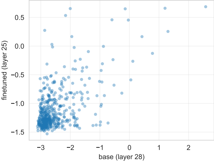
TriviaMC: base vs finetuned Spearman \rho = 0.811 ( p=3.96e-188 )
