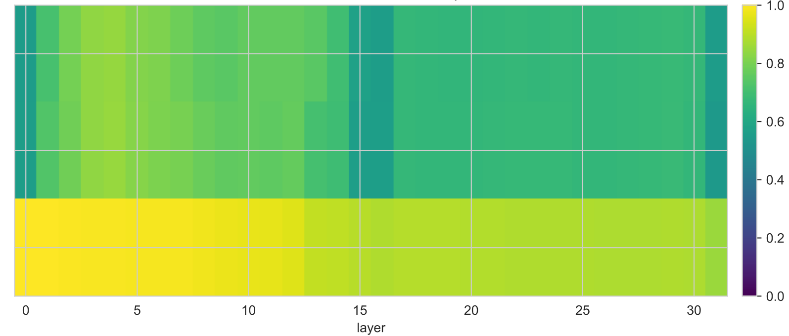
TriviaMC — cross-model RSM Spearman
