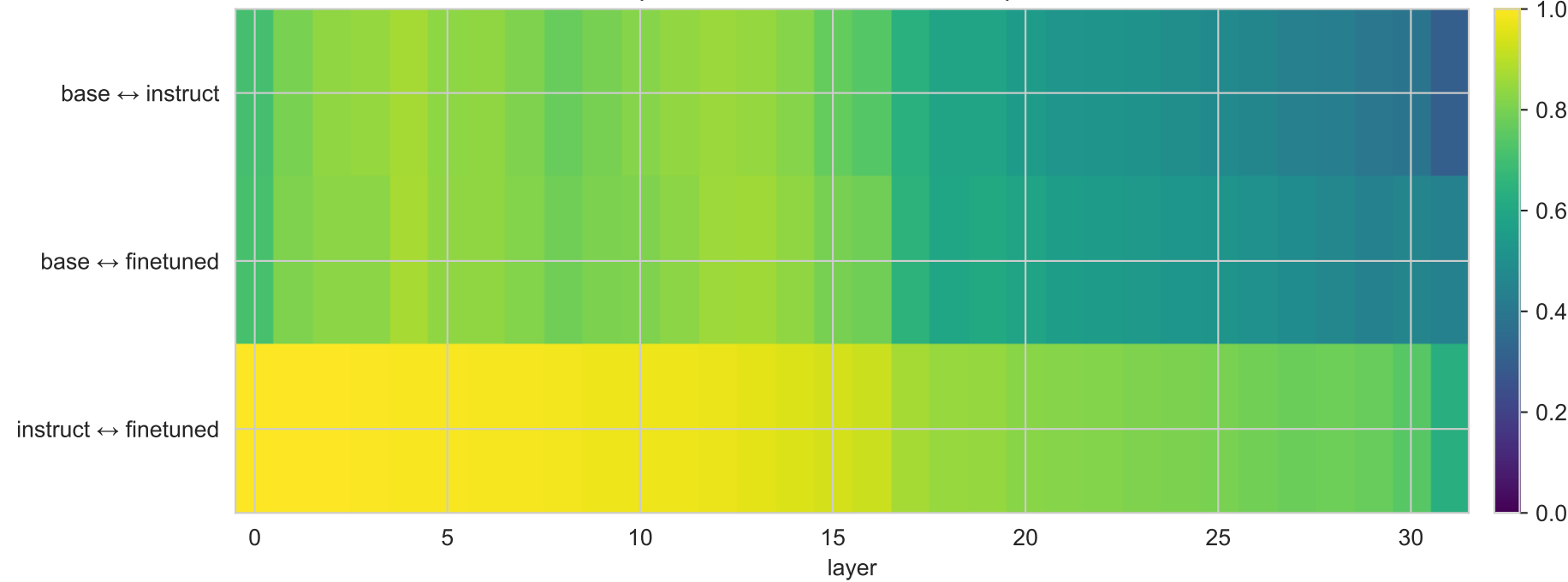
SimpleMC — cross-model RSM Spearman
