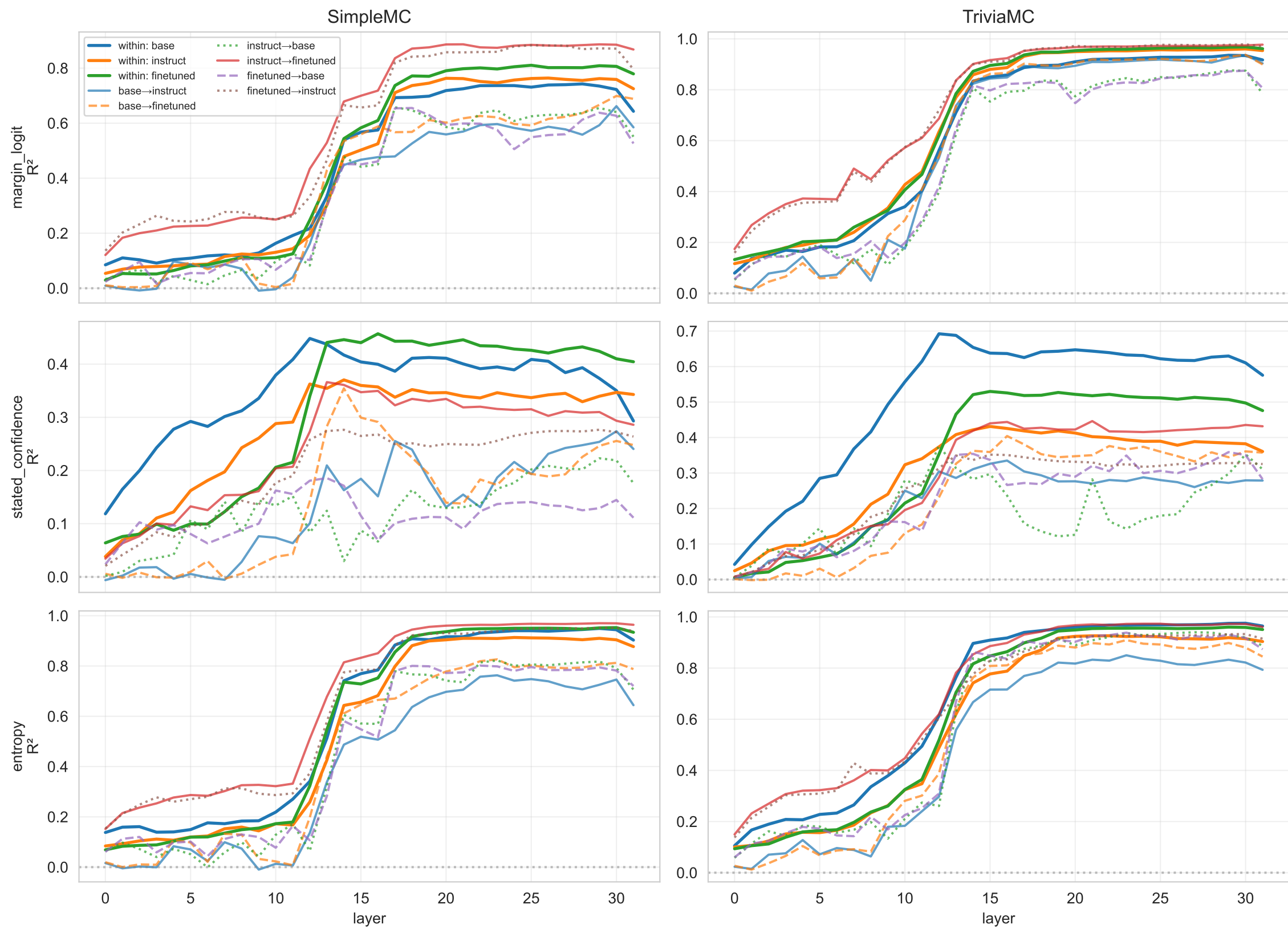
Cross-model probe R^2 (solid = within-model, dashed/dotted = cross-model)
