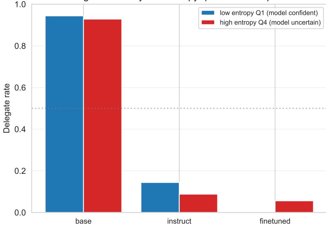
Delegation rate by MC-entropy quartile — SimpleMC
