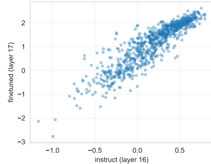
TriviaMC: instruct vs finetuned Spearman \rho = 0.911 ( p=1.74e-308 )
