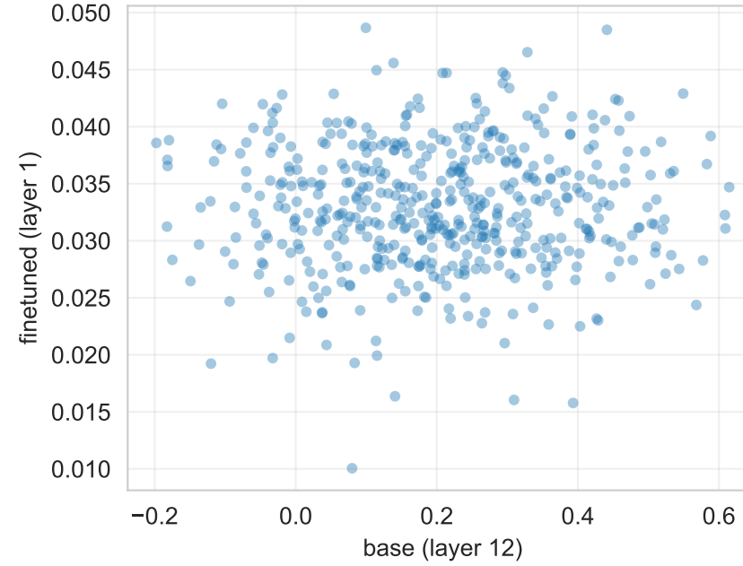
TriviaMC: base vs finetuned Spearman \rho = 0.635 ( p=3.18e-31 )
