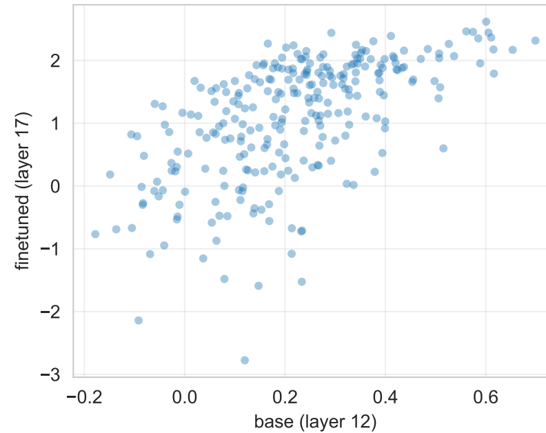
TriviaMC: base vs finetuned Spearman \rho = 0.635 ( p=3.18e-31 )
