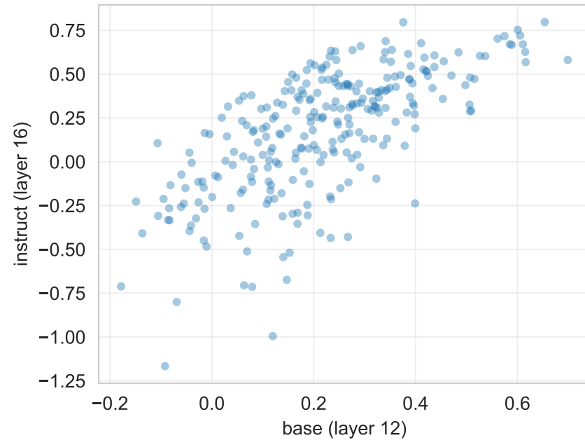
TriviaMC: base vs instruct Spearman \rho = 0.697 ( p=1.07e-39 )
