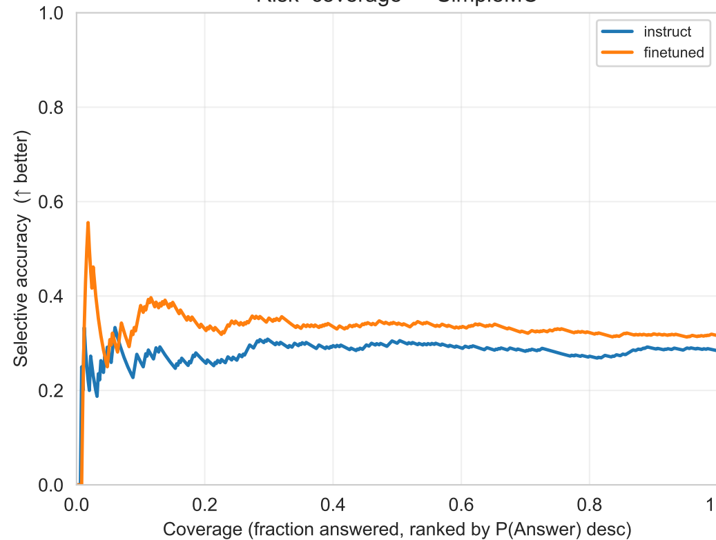
Risk-coverage — SimpleMC
