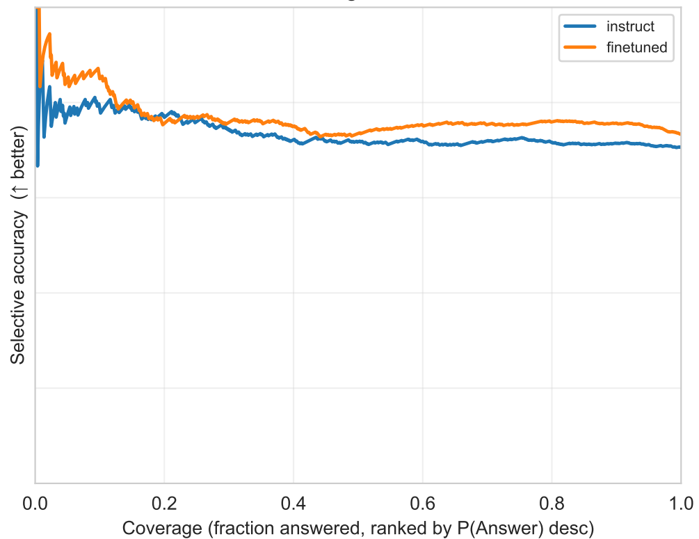
Risk-coverage — TriviaMC
