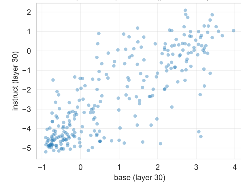
TriviaMC: base vs instruct Spearman \rho = 0.790 ( p=1.12e-57 )
