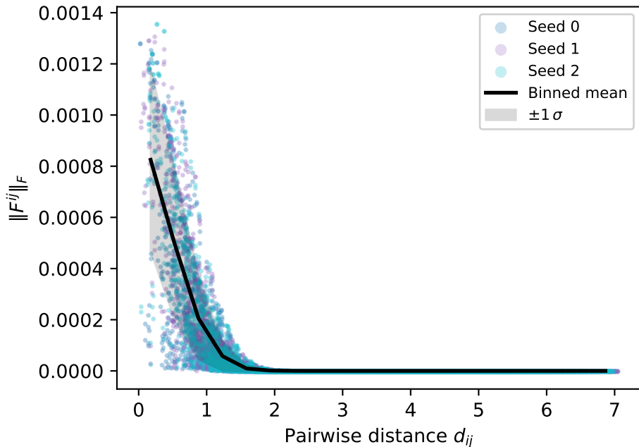
Sensitivity block norm vs. agent distance (Vicsek, N = 125 , r = 0.5 , T = 5 )
