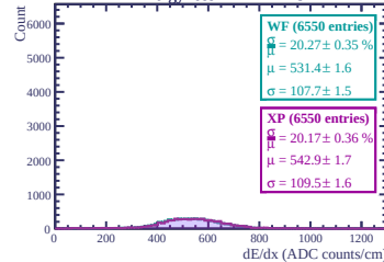
Energy loss in ERAM 36
