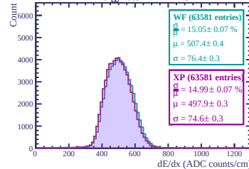
Energy loss in ERAM 7
