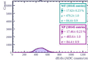
Energy loss in ERAM 46
