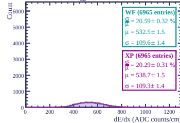
Energy loss in ERAM 37
