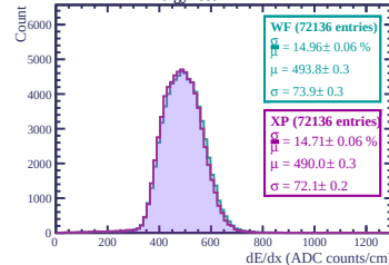
Energy loss in ERAM 41
