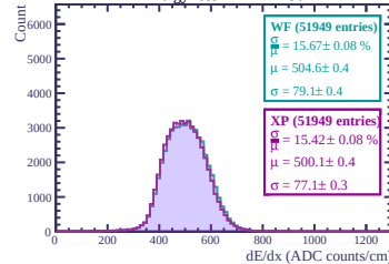
Energy loss in ERAM 44
