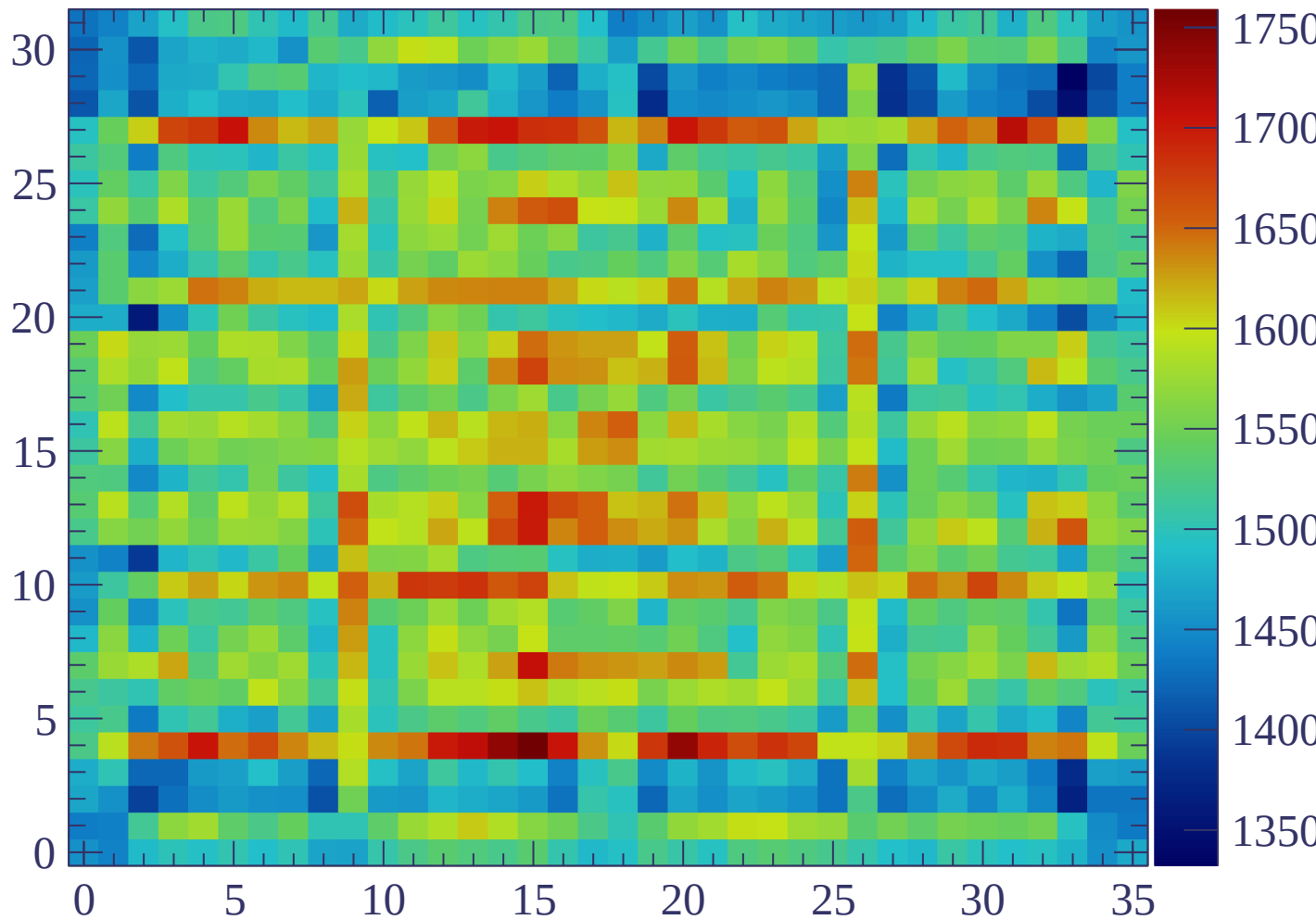
Average gain map
