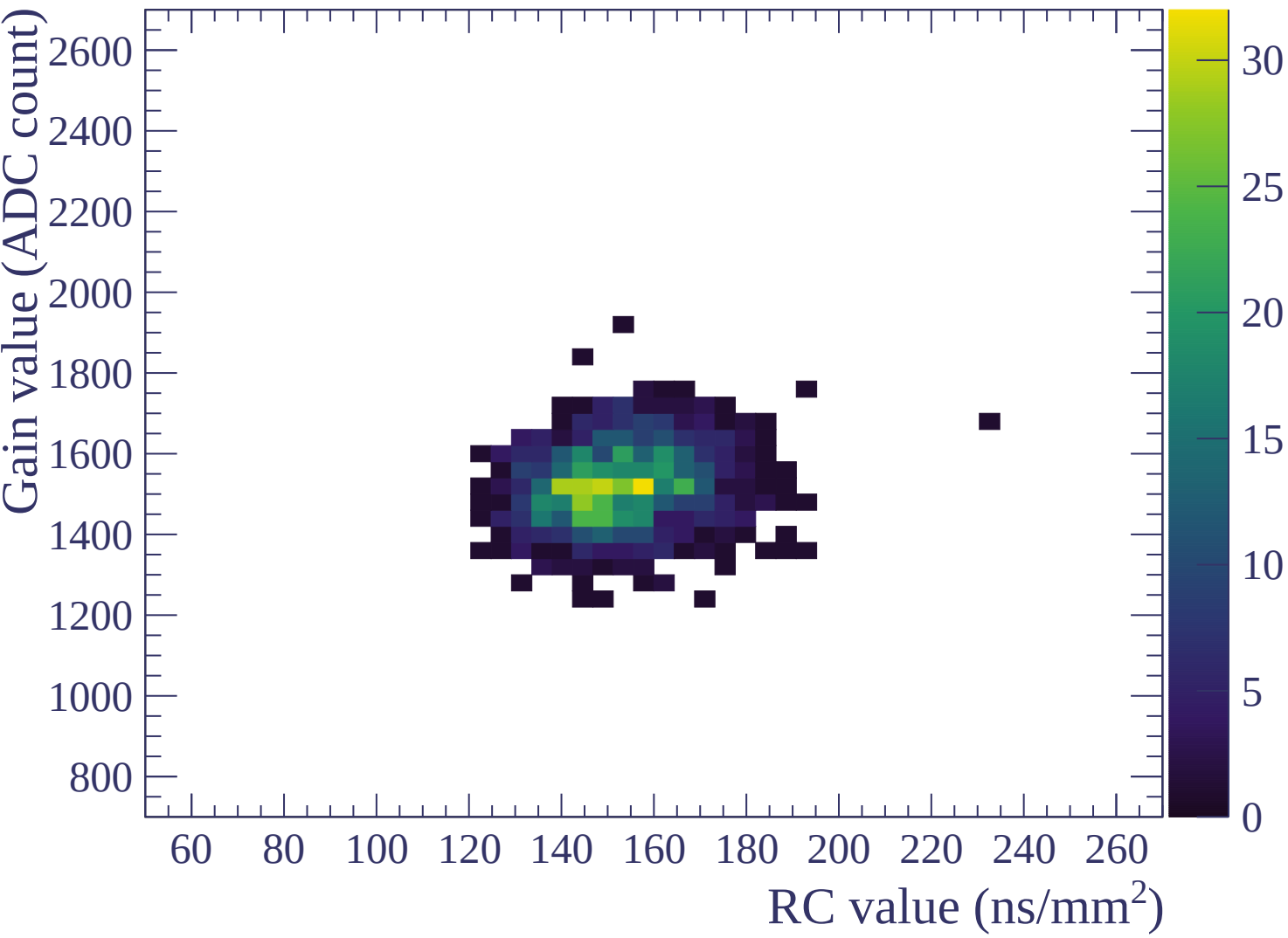
ERAM#46 Gain vs RC
