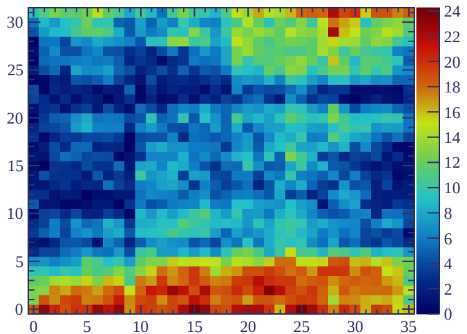
Absolute difference of tHAT vs bHAT normalized average RC map (in %)
