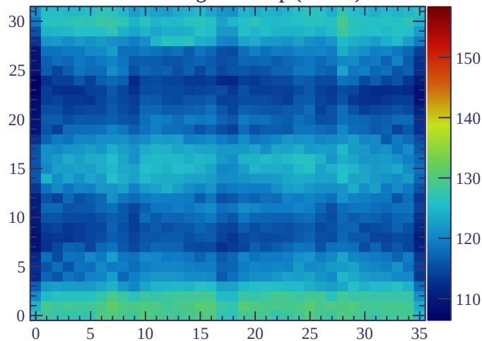
Average RC map (bHAT)
