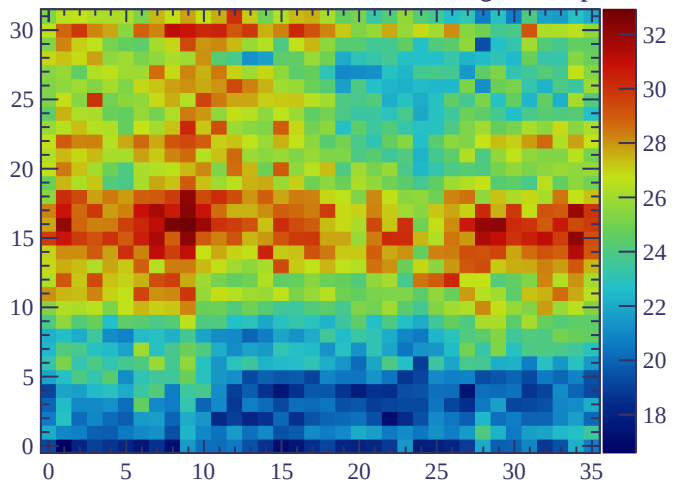
Difference of tHAT vs bHAT average RC map
