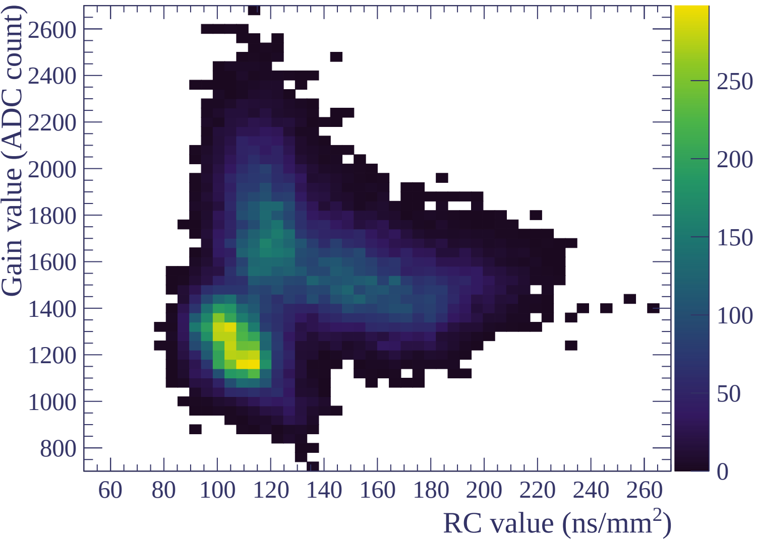
Gain vs RC
