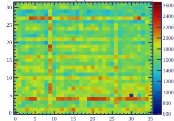
ERAM#10 (13) Gain = 1700
