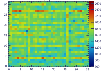
ERAM#36 (23) Gain = 1609
