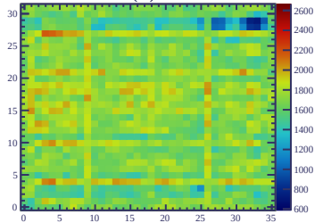
ERAM#45 (21) Gain = 1540
