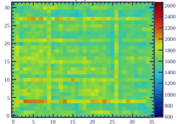
ERAM#12 (32) Gain = 1639
