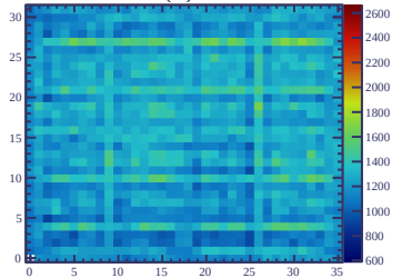
ERAM#37 (22) Gain = 1679
