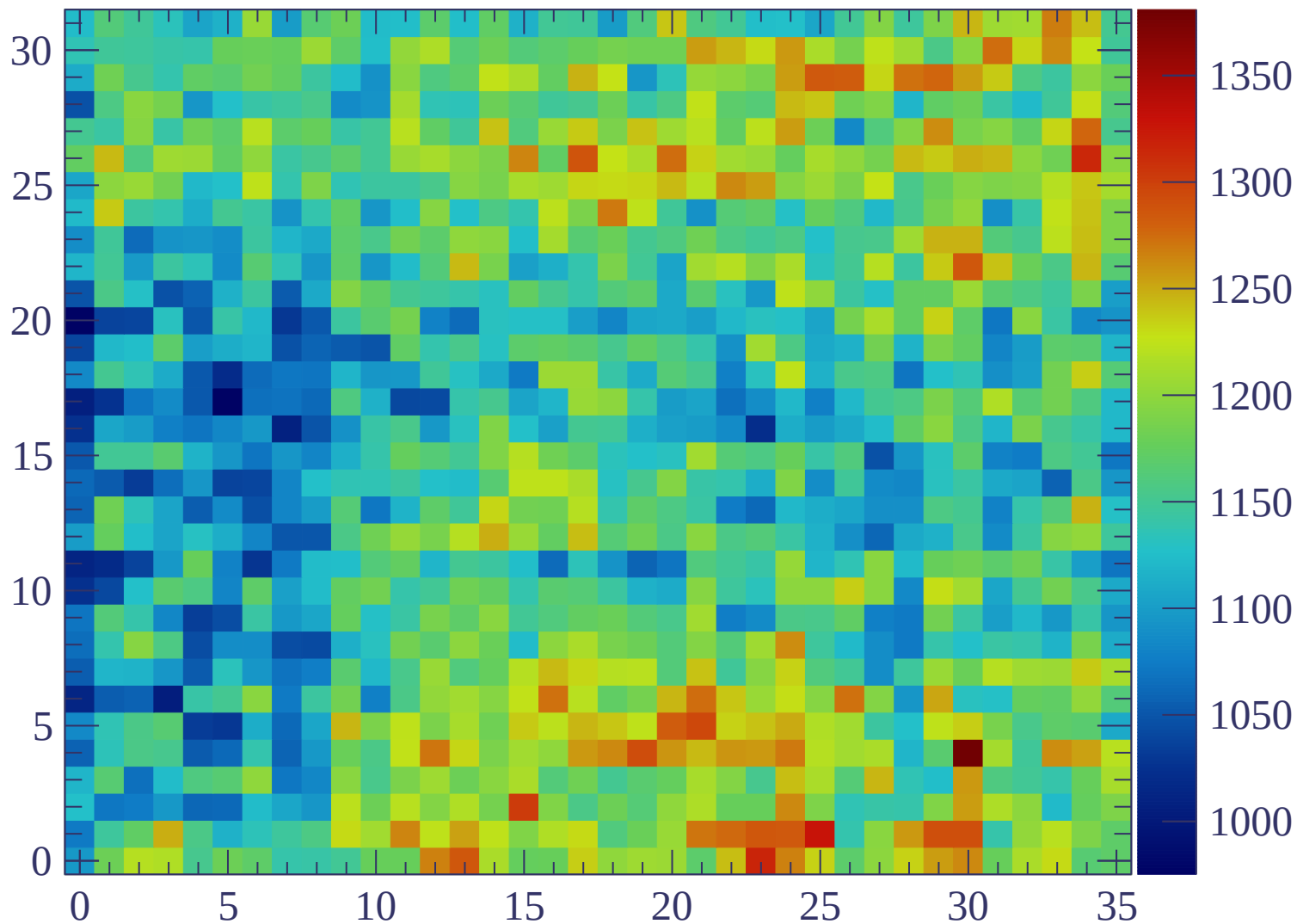
ERAM#28 (2) Gain = 1158
