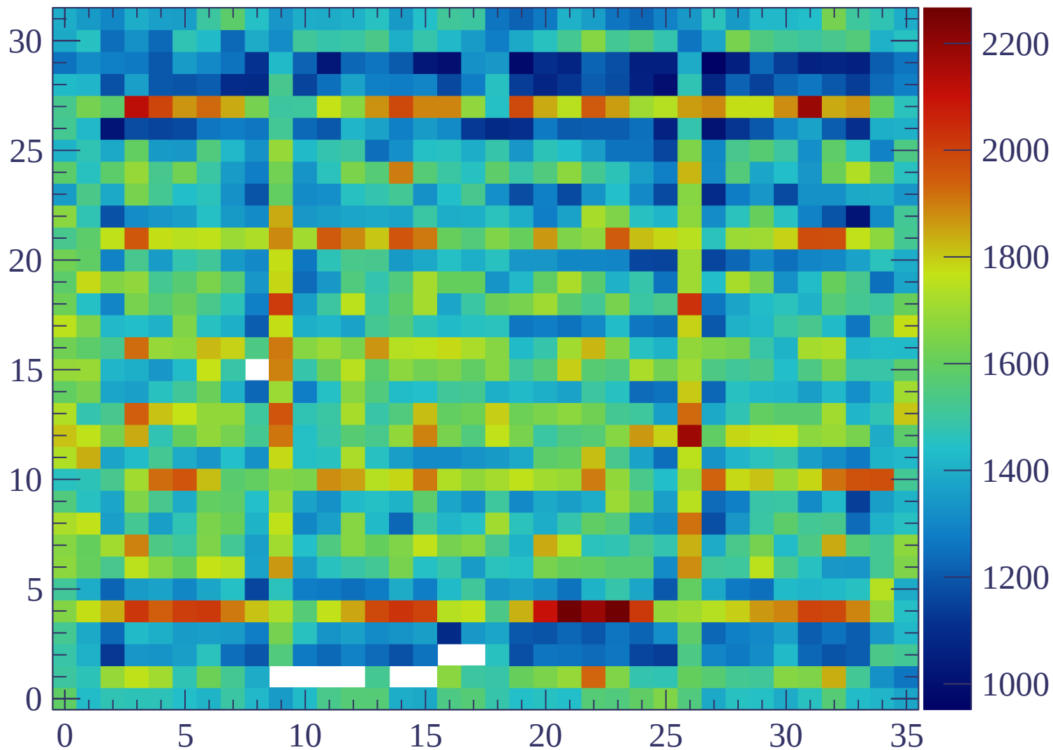
ERAM#9 (6) Gain = 1485
