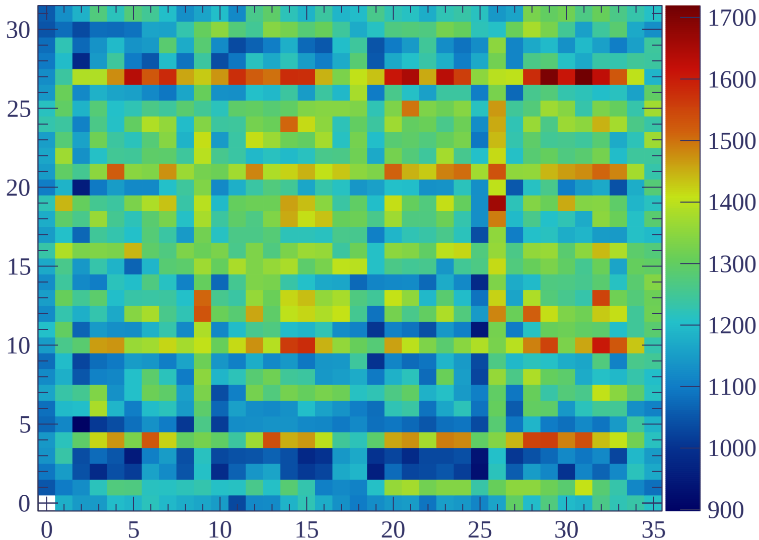
ERAM#14 (18) Gain = 1243
