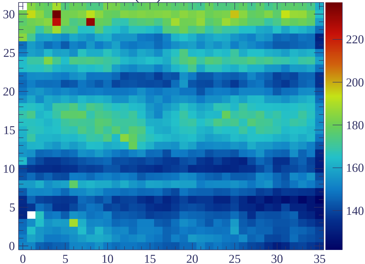
ERAM#41 (30) RC = 155 ns/mm 2
