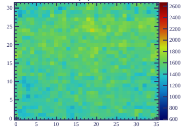
ERAM#46 (31) Gain = 1523
