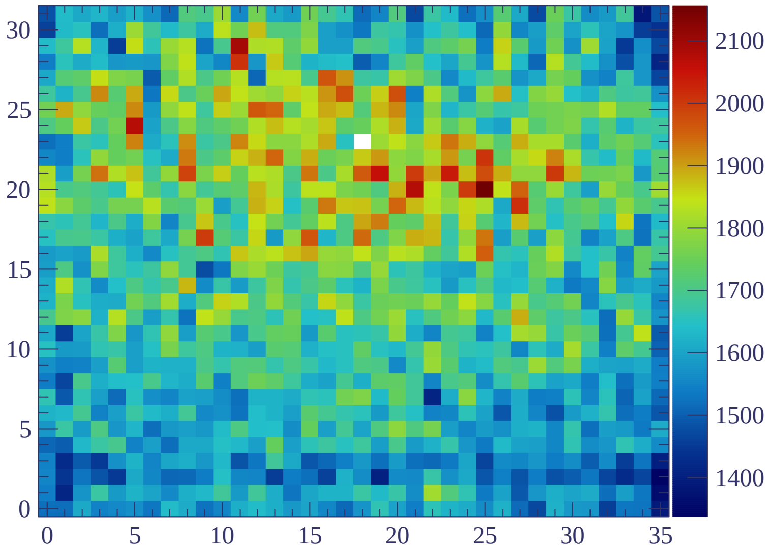
ERAM#37 (22) Gain = 1679
