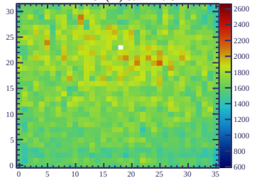
ERAM#7 (26) Gain = 1901
