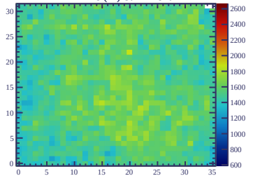
ERAM#38 (25) Gain = 1524
