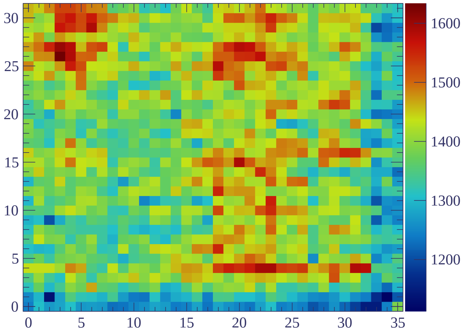
ERAM#23 (10) Gain = 1393
