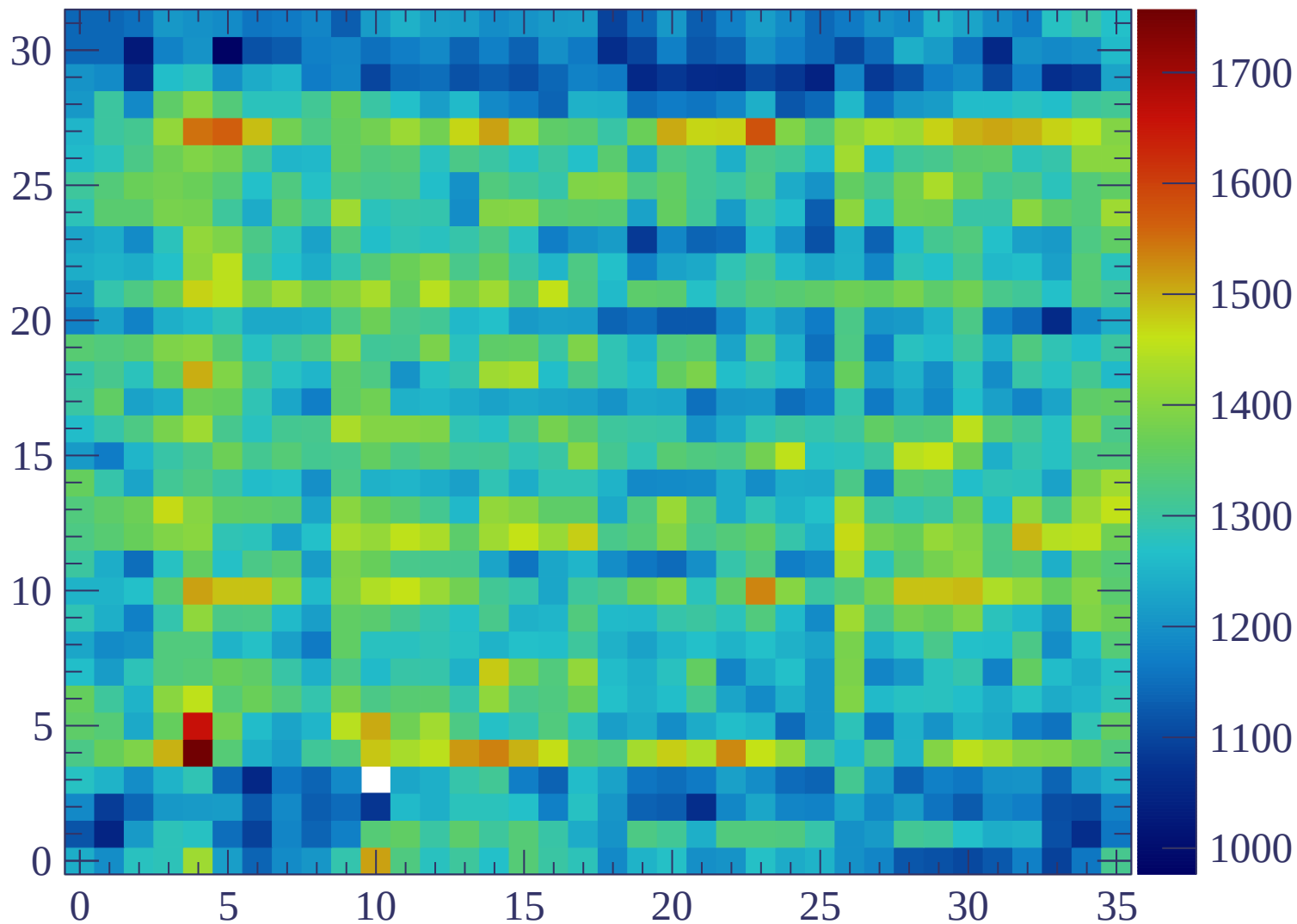
ERAM#21 (4) Gain = 1283
