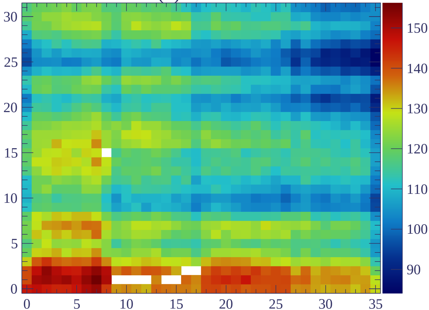
ERAM#9 (6) RC = 116 ns/mm 2
