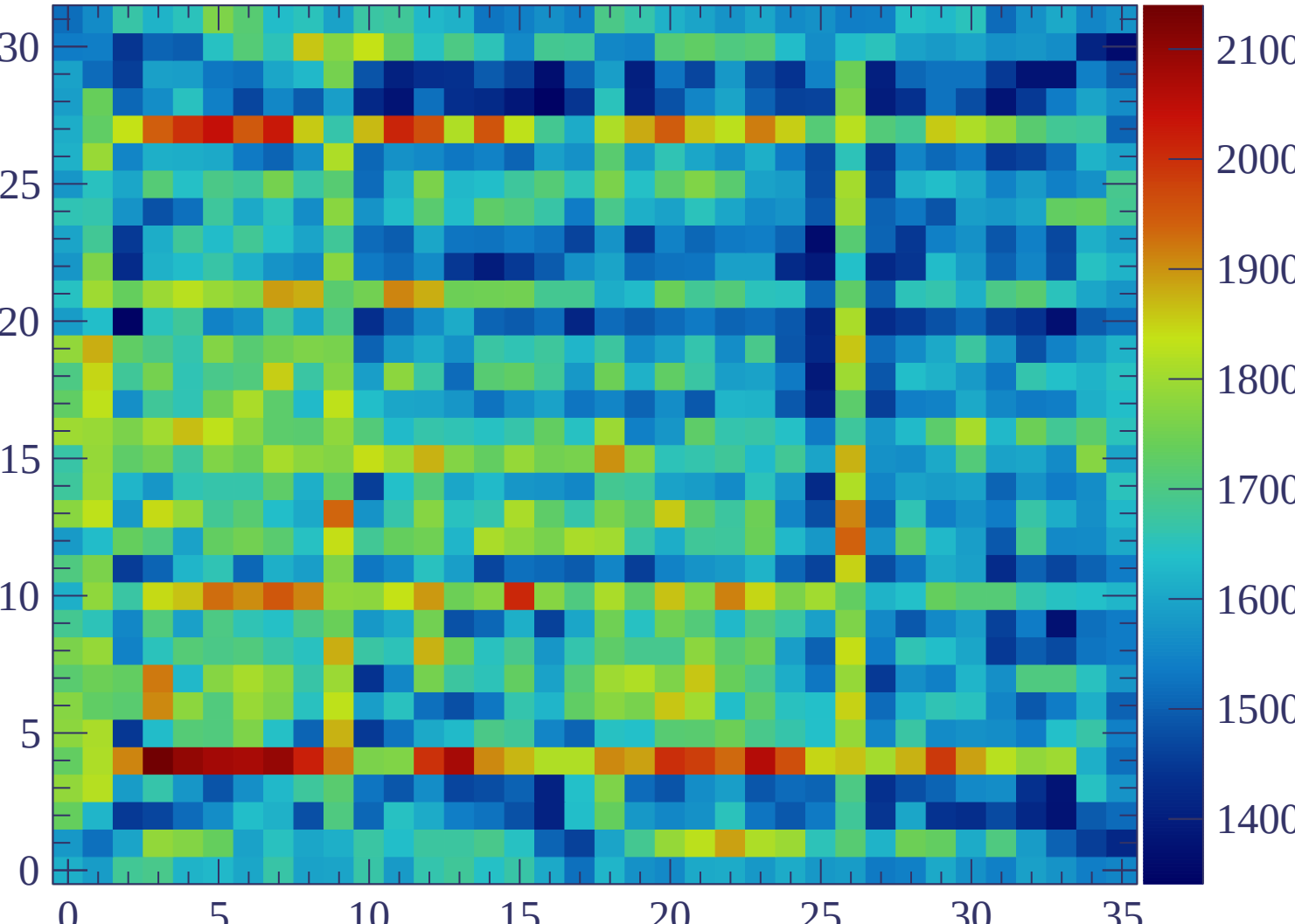
ERAM#12 (32) Gain = 1639
