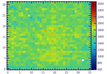
ERAM#39 (29) Gain = 1647
