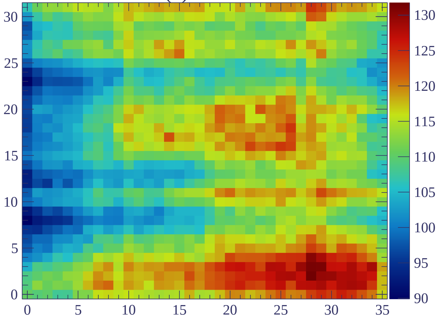
ERAM#30 (1) RC = 112 ns/mm 2
