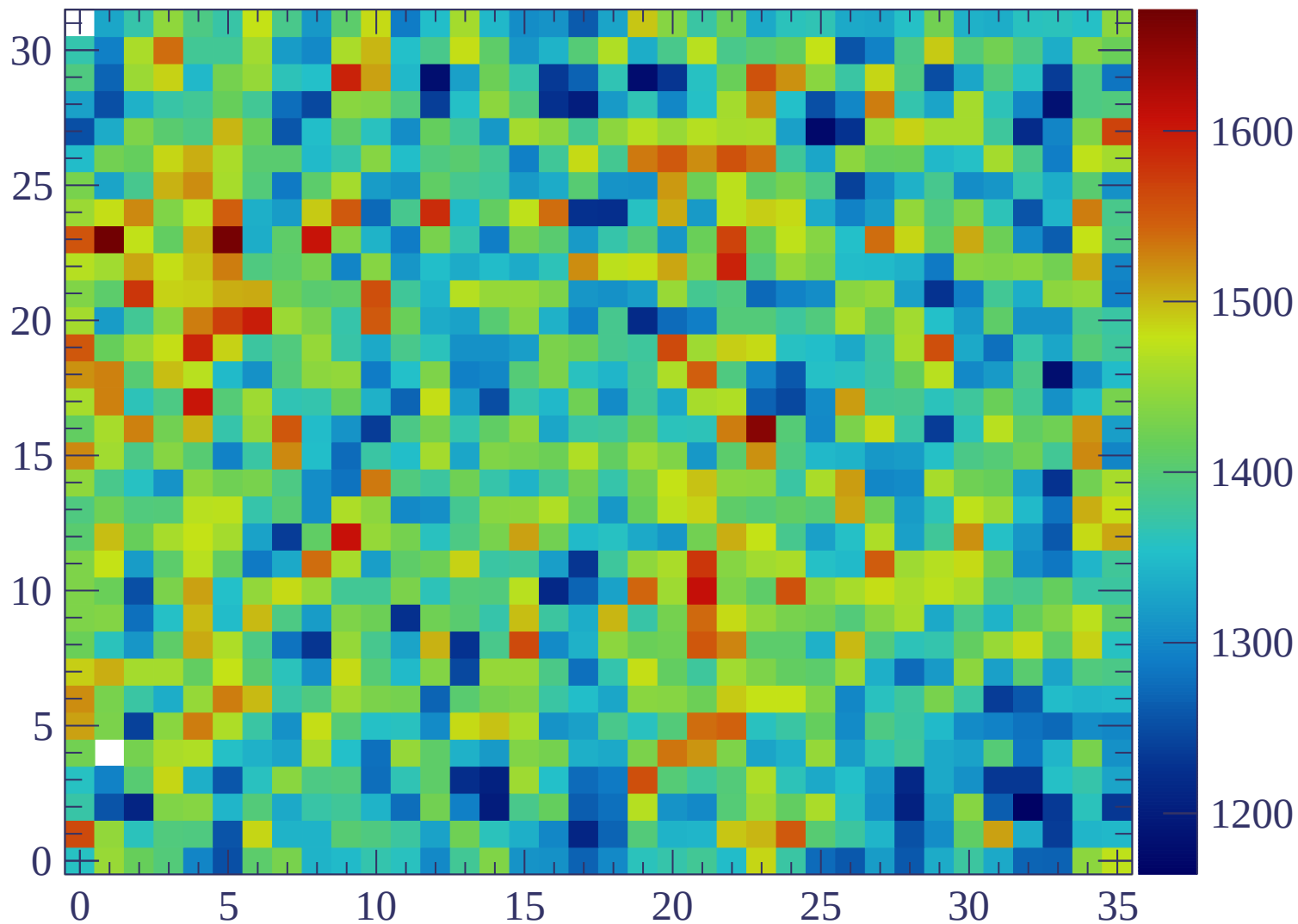
ERAM#41 (30) Gain = 1390
