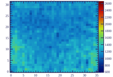
ERAM#1 (12) Gain = 1946
