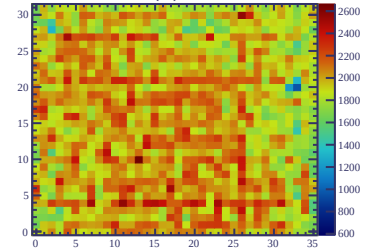
ERAM#3 (15) Gain = 1984
