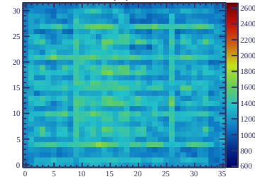
ERAM#18 (33) Gain = 1283
