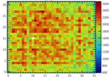
ERAM#15 (19) Gain = 1629
