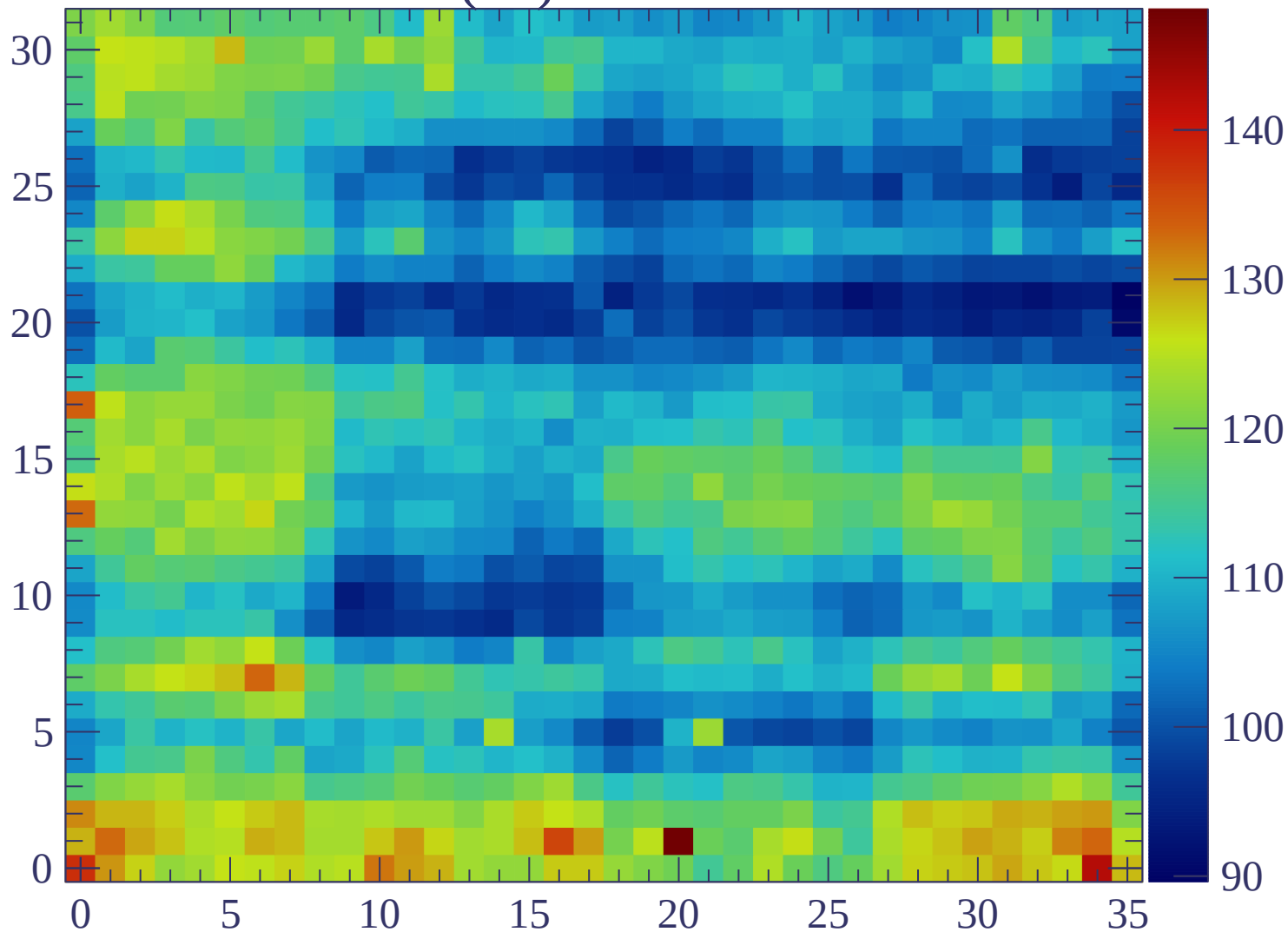
ERAM#7 (26) RC = 111 ns/mm 2
