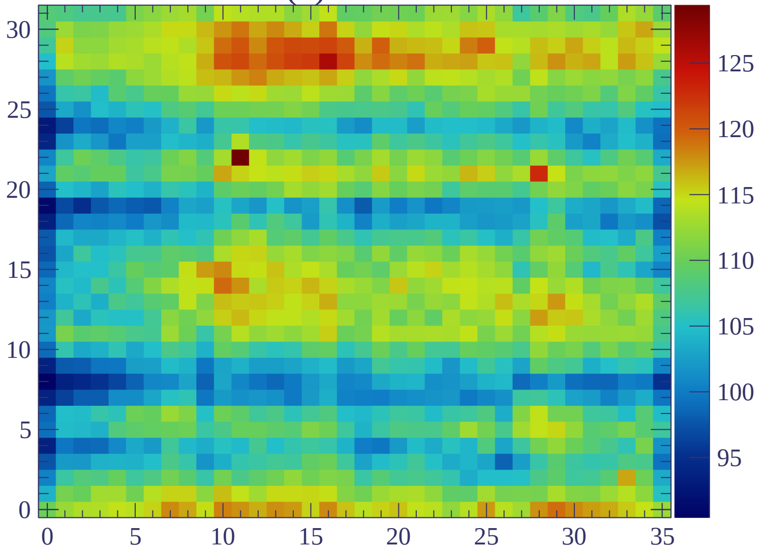
ERAM#19 (3) RC = 109 ns/mm 2
