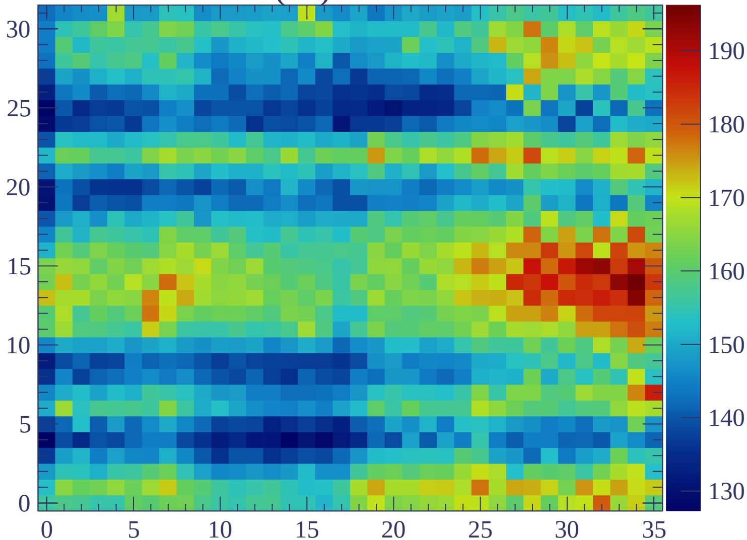
ERAM#39 (29) RC = 155 ns/mm 2
