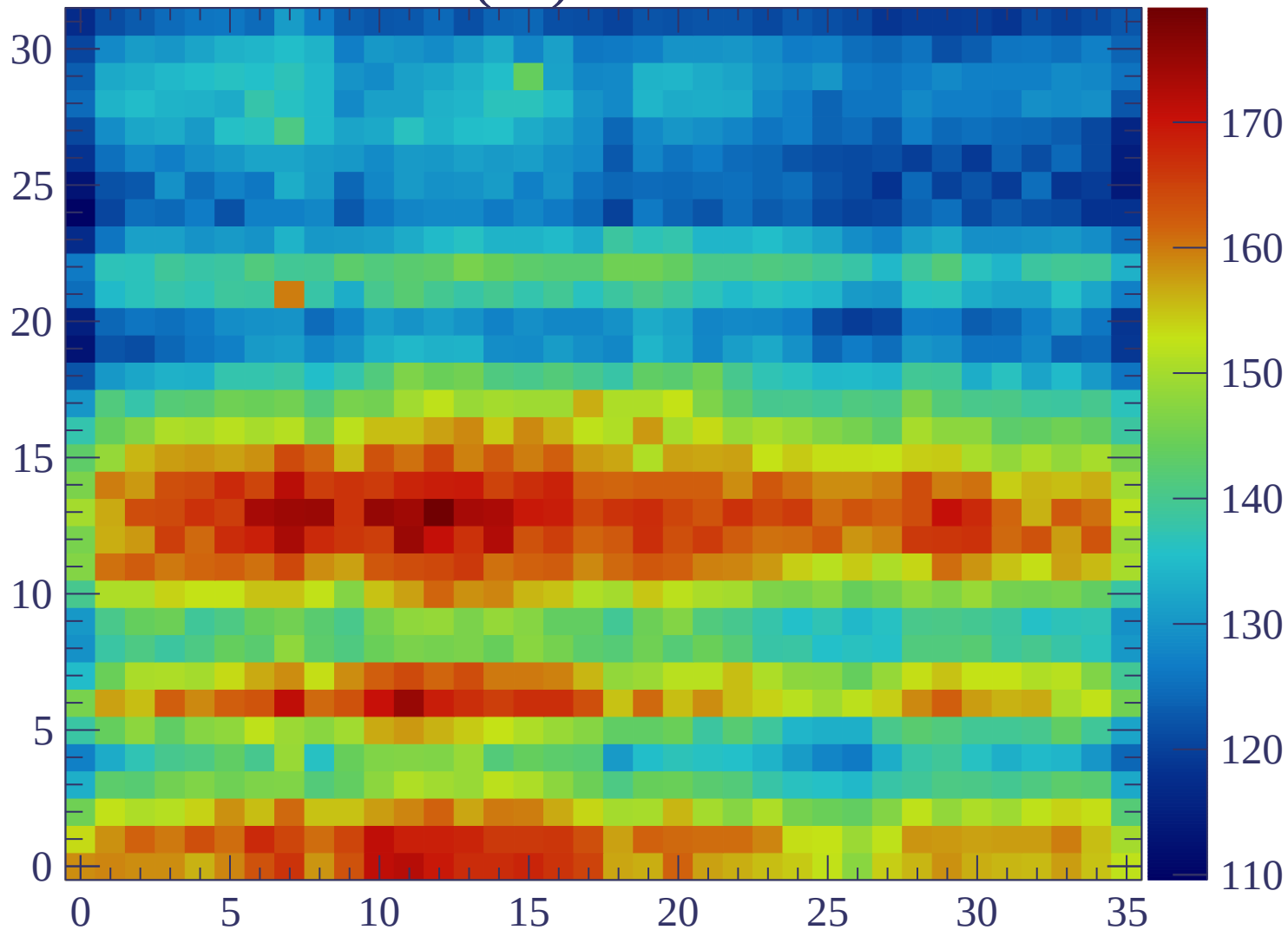
ERAM#12 (32) RC = 142 ns/mm 2
