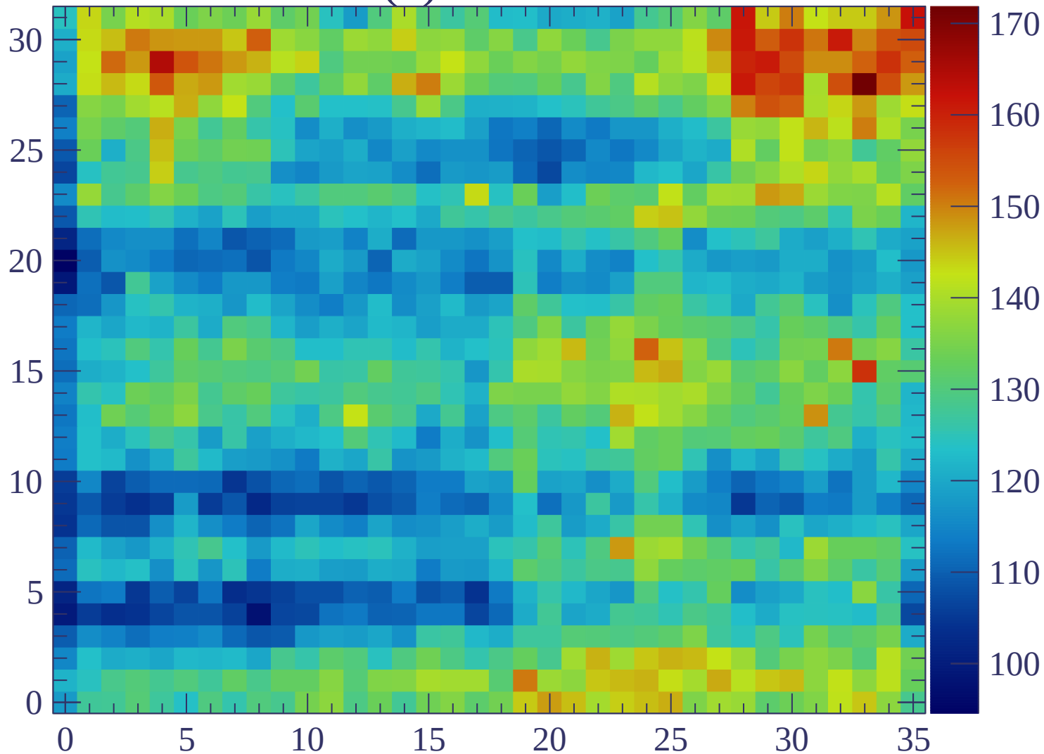
ERAM#2 (7) RC = 127 ns/mm 2
