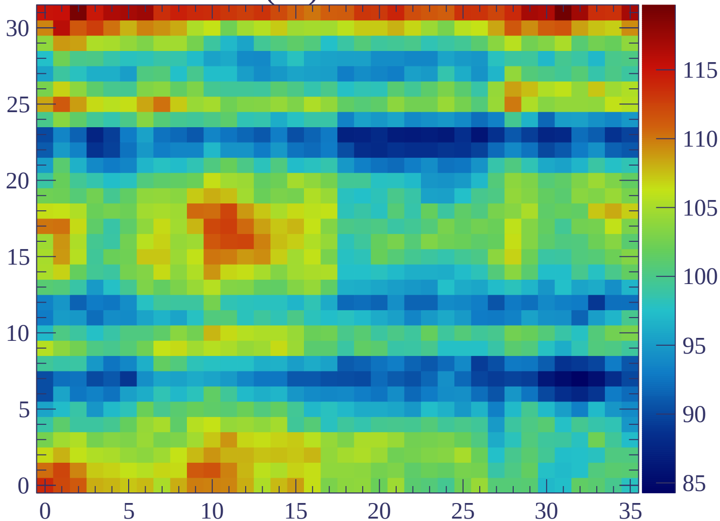
ERAM#29 (11) RC = 100 ns/mm 2
