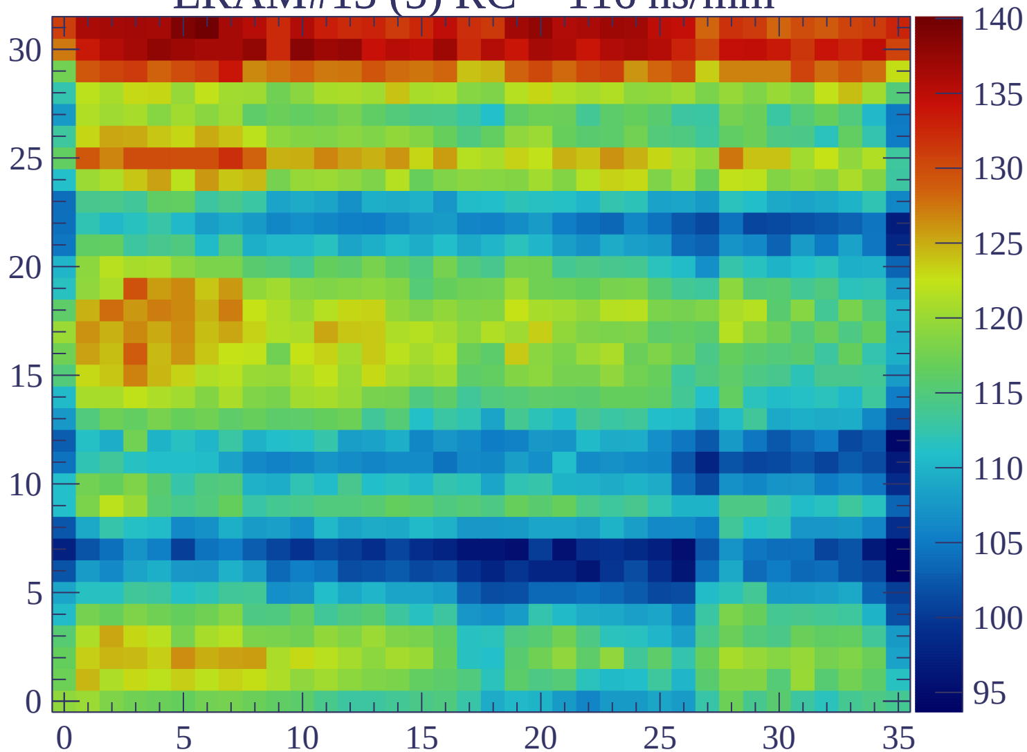
ERAM#13 (5) RC = 116 ns/mm 2
