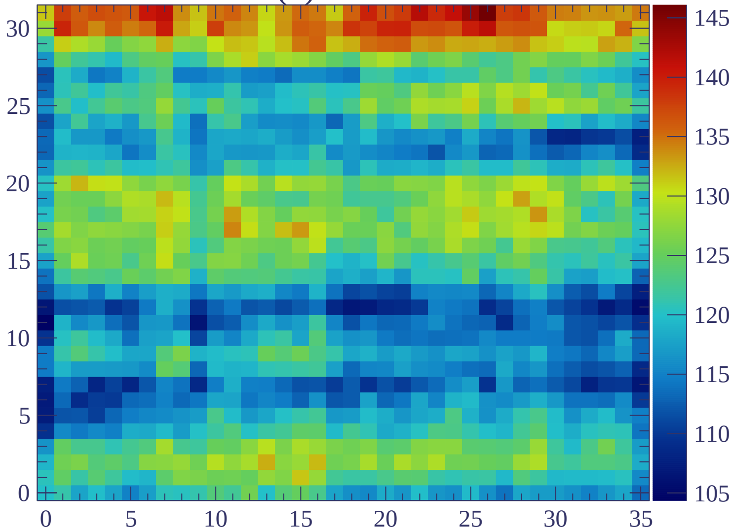
ERAM#17 (9) RC = 122 ns/mm 2
