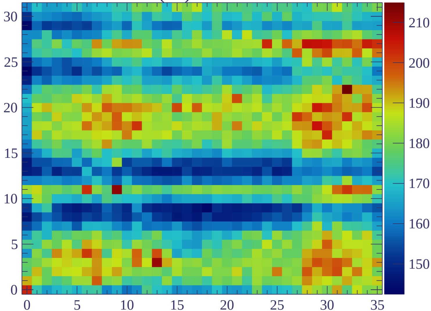
ERAM#42 (20) RC = 174 ns/mm 2
