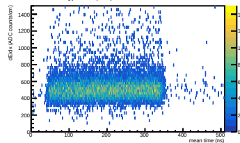
Energy loss (WF) vs mean time in ERAM 9
