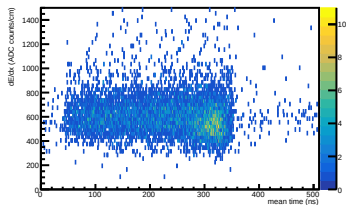
Energy loss (WF) vs mean time in ERAM 1
