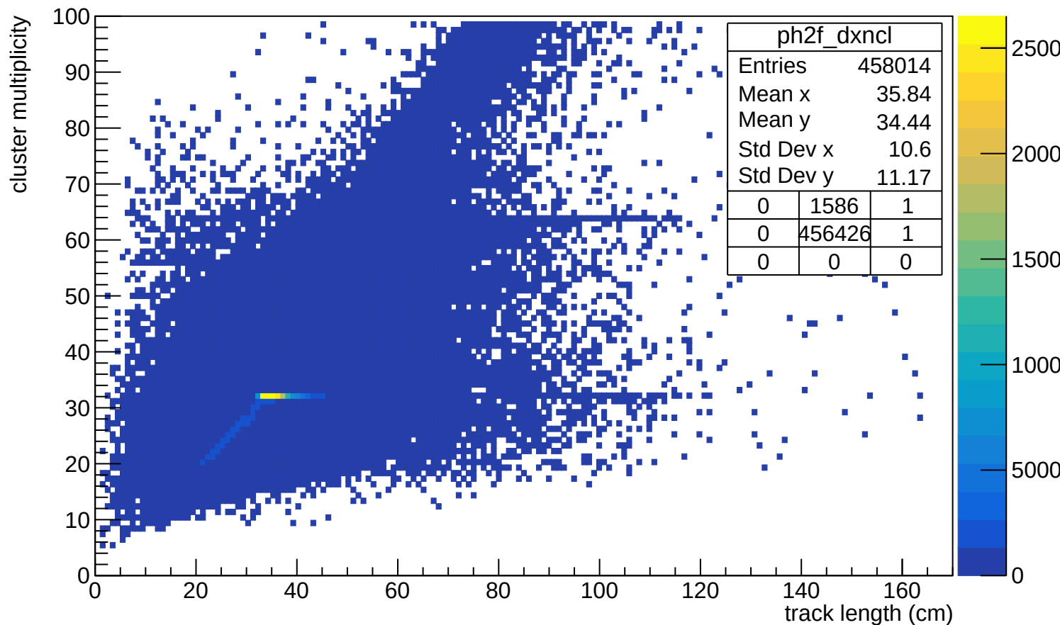
Track length vs cluster multiplicity
