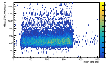
Energy loss (WF) vs mean time in ERAM 23
