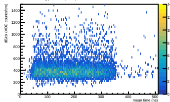
Energy loss (WF) vs mean time in ERAM 30
