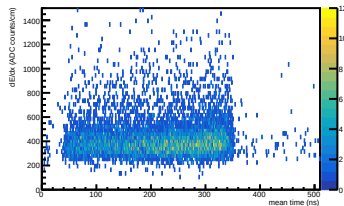
Energy loss (WF) vs mean time in ERAM 17
