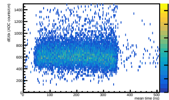
Energy loss (WF) vs mean time in ERAM 3
