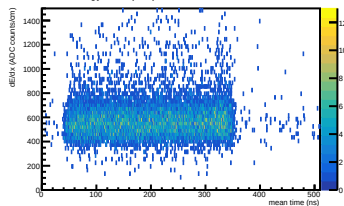
Energy loss (WF) vs mean time in ERAM 13
