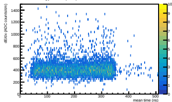
Energy loss (WF) vs mean time in ERAM 21
