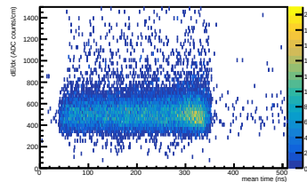
Energy loss (WF) vs mean time in ERAM 11
