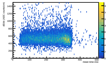
Energy loss (WF) vs mean time in ERAM 10
