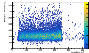
Energy loss (WF) vs mean time in ERAM 29
