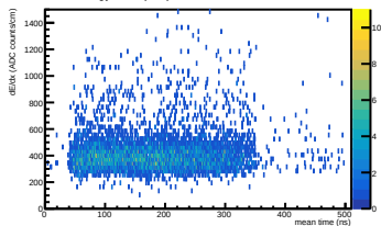
Energy loss (WF) vs mean time in ERAM 24
