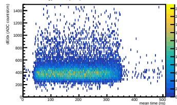
Energy loss (WF) vs mean time in ERAM 28
