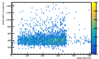
Energy loss (WF) vs mean time in ERAM 26
