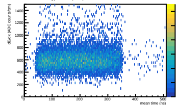
Energy loss (WF) vs mean time in ERAM 2
