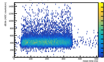
Energy loss (WF) vs mean time in ERAM 19
