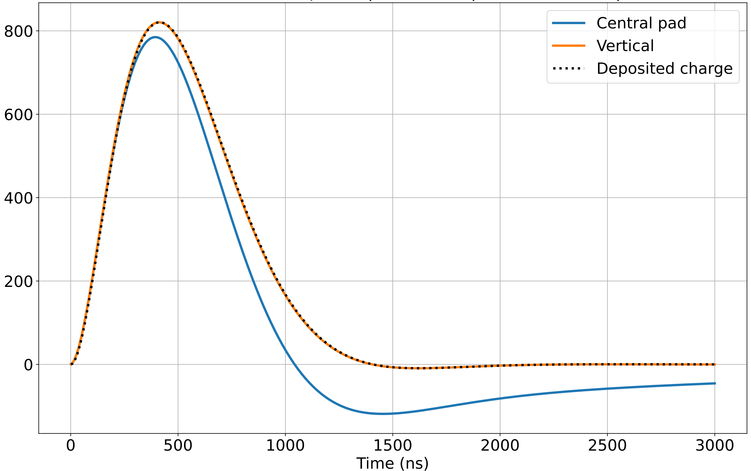
Normalized dE/dx for clusters ( \varphi=0.0^\circ | d=-0.0 mm | RC=120 ns/mm 2 | z=250 mm)
