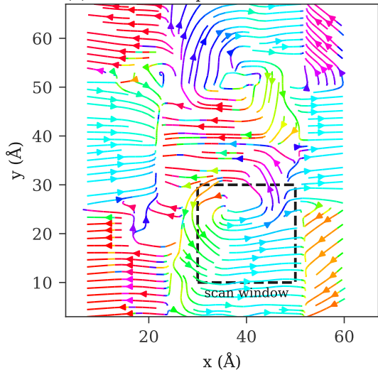
(a) ferroelectric polar domains
