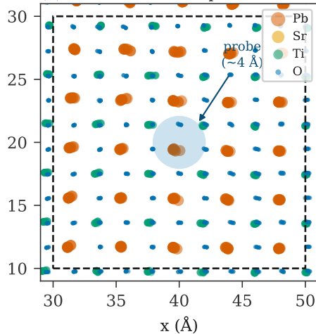
(b) atomic columns + probe
