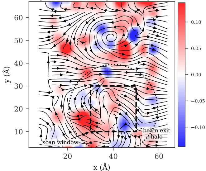
(a) polar domains + acquisition footprint
