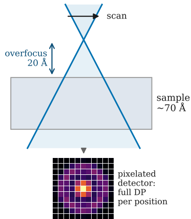
(a) 4D-STEM acquisition
