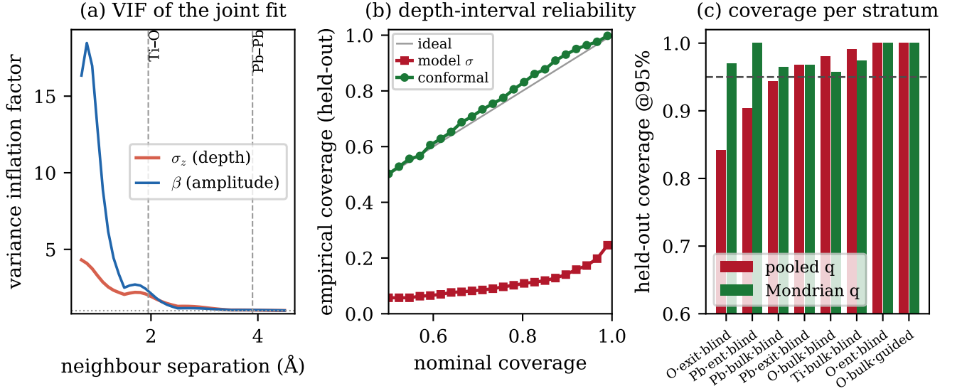
FIG. 3. Calibrated uncertainty, from a 50/50 split-conformal calibration/test split. (a) Variance inflation factor (VIF) of the joint fit against neighbour separation: near unity at the 3.9 \text{ Å} heavy-atom spacing, \approx 2 in depth at the 1.95 \text{ Å} Ti-O spacing. (b) Held-out reliability of the depth interval: the raw model standard error treated as Gaussian (red) severely under-covers, whereas the conformal interval (blue) tracks the ideal diagonal. (c) Held-out coverage at 95% for the eight strata where a pooled quantile (red squares) departs most from target; the label-conditional quantile (blue circles) restores each.
