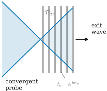
(a) multislice propagation potential slices
