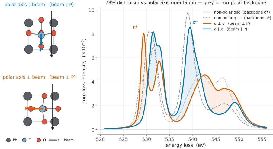
FIG. 5. Orientation dichroism of the PbTiO 3 apical-oxygen O K edge from core-hole CASTEP and OptaDOS. With the momentum transfer across the polar axis ( \mathbf{q} \perp c , beam \perp \mathbf{P} ) the edge shows a sharp \pi^* peak; along it ( \mathbf{q} \parallel c , beam \parallel \mathbf{P} ) it shows the \sigma^* features of the O 2p_z states directed along the Ti-O-Ti chain. Grey curves are the same two orientations for the zero-polarisation, non-polar and equally strained reference, isolating the backbone contribution.
