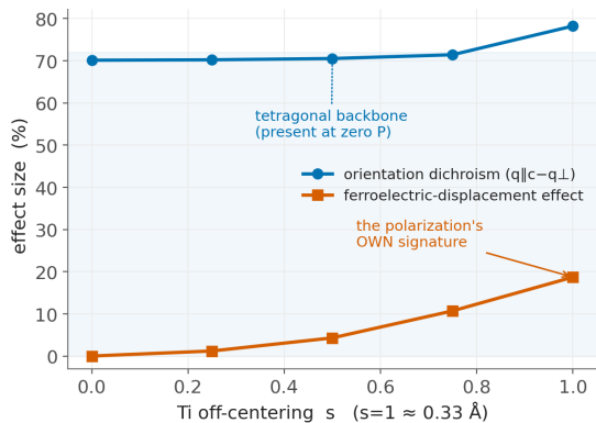
FIG. 6. Separating strain from polarisation. Holding the lattice parameters fixed and varying only the internal Ti off-centering s , the total orientation dichroism (blue) is already 70% at zero polarisation, corresponding to the tetragonal backbone, whereas the signature of the ferroelectric displacement itself (orange) grows monotonically to 19% at the experimental off-centring |u| \approx 0.33 \text{ \AA} .
