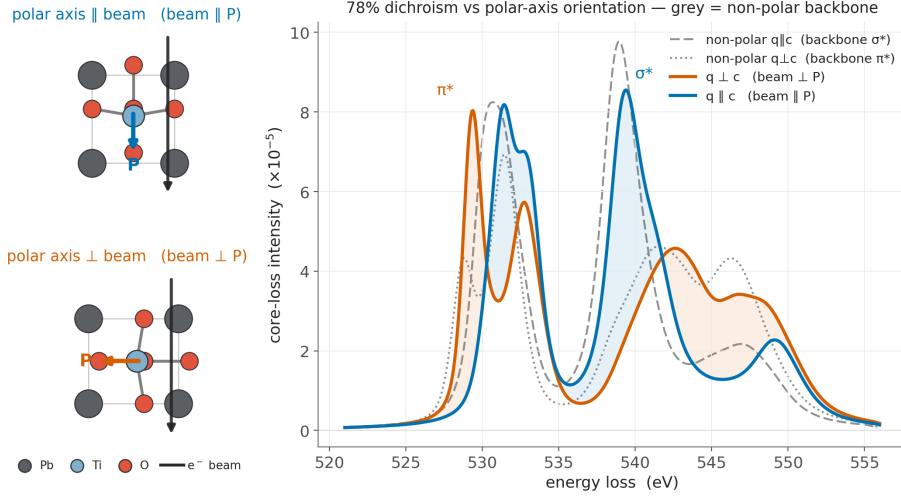
FIG. 5. Orientation dichroism of the \text{PbTiO}_3 apical-oxygen O K edge from core-hole CASTEP and OptaDOS. With the momentum transfer across the polar axis ( \mathbf{q} \perp \mathbf{c} , beam \perp \mathbf{P} ) the edge shows a sharp \pi^* peak; along it ( \mathbf{q} \parallel \mathbf{c} , beam \parallel \mathbf{P} ) it shows the \sigma^* features of the O 2p_z states directed along the Ti–O–Ti chain. Grey curves are the same two orientations for the zero-polarisation, non-polar and equally strained reference, isolating the backbone contribution.
