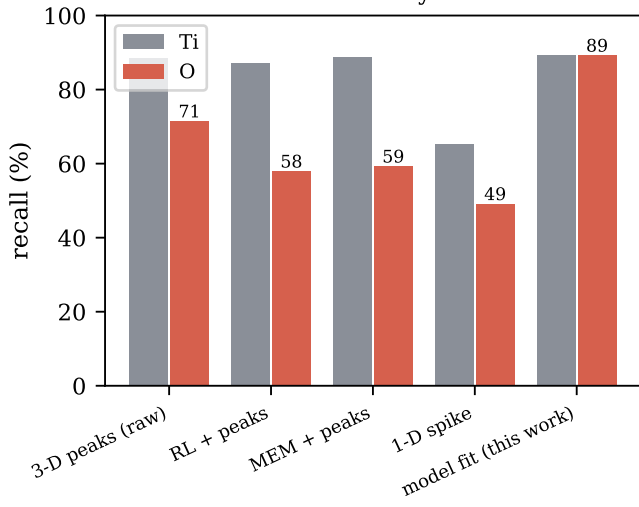
Ti and O recall by method
