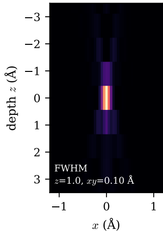
(a) measured PSF K
