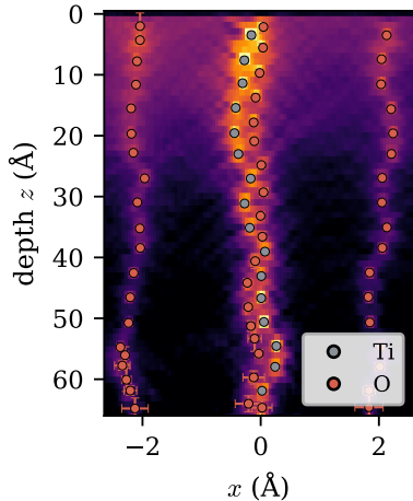
(b) forward model on a B-O column (c) blind atoms + 95% interval
