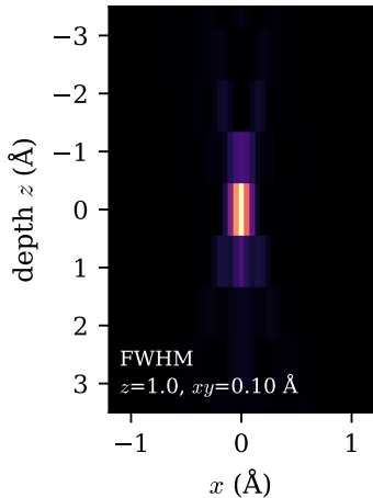
(a) measured PSF K
