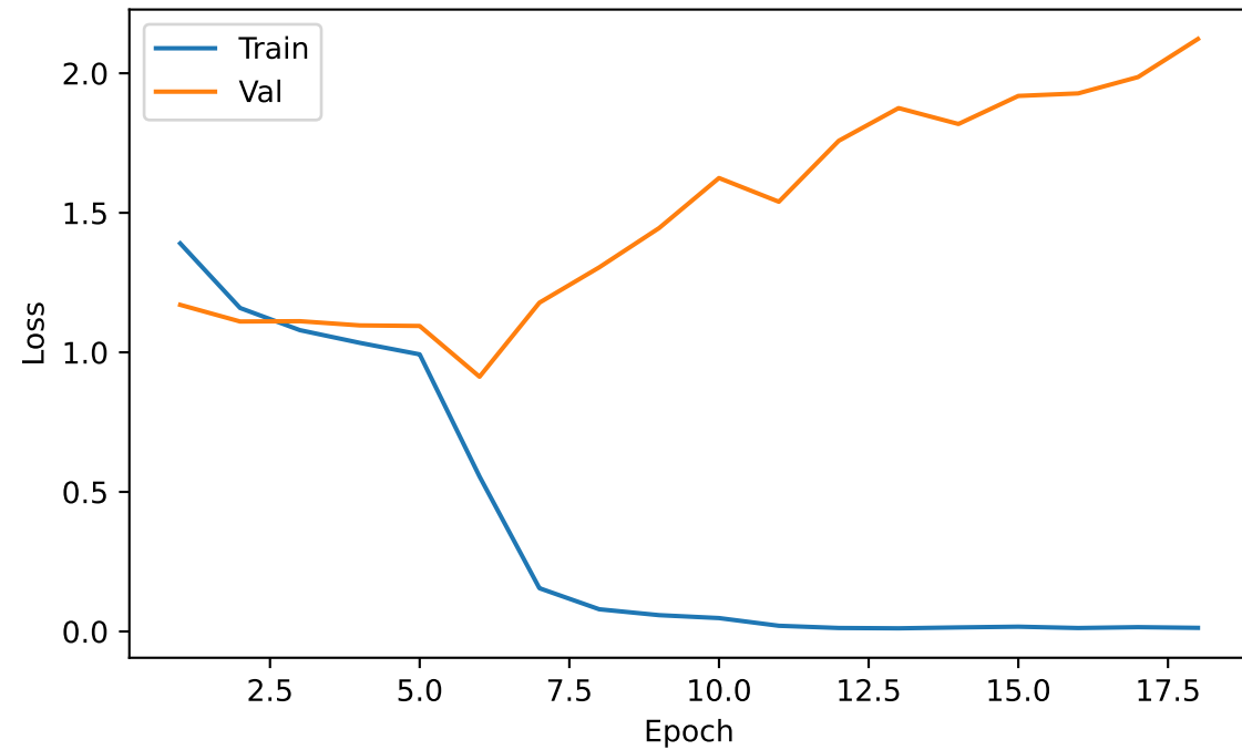
Stage 1 (Mel + Frozen ResNet-18) — Loss
