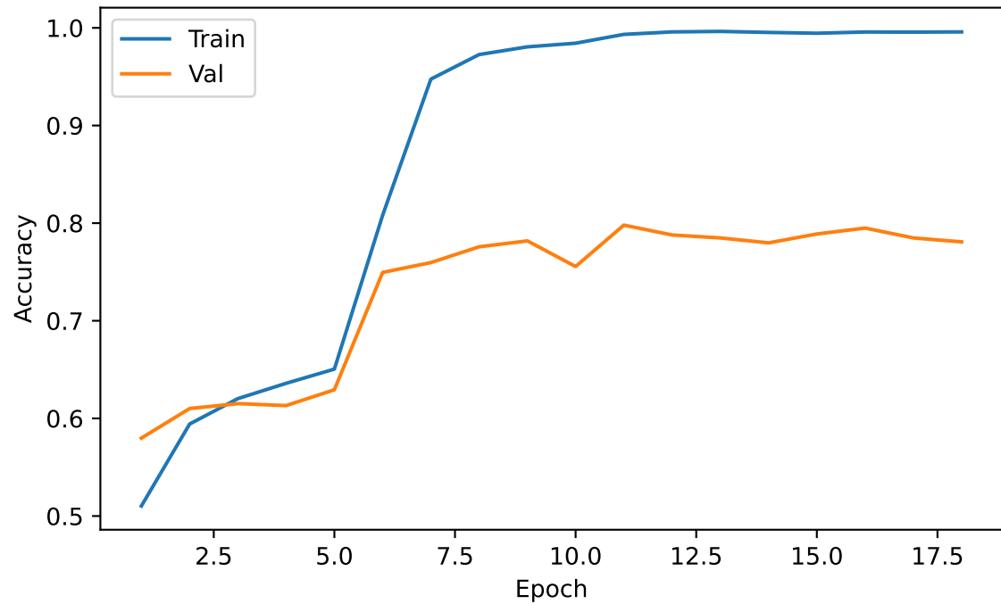
Stage 1 (Mel + Frozen ResNet-18) — Accuracy
