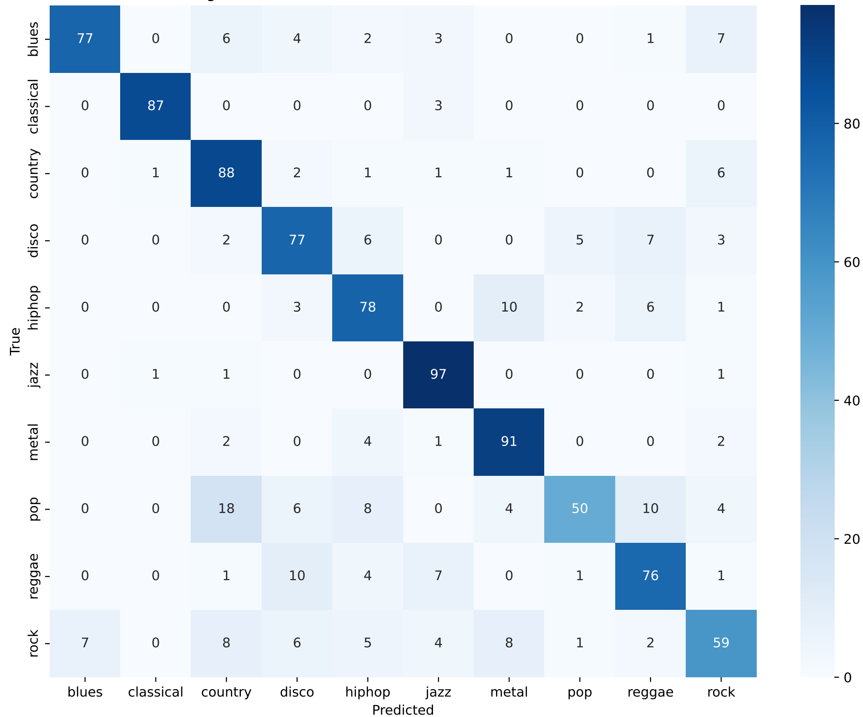
Stage 2 (3-Branch Fusion) — Confusion Matrix (Test Set)
