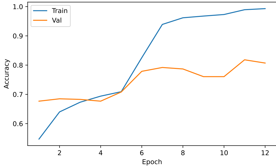
Stage 2 (3-Branch Fusion) — Accuracy
