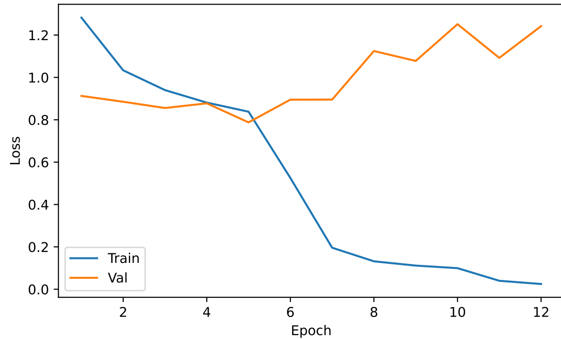
Stage 2 (3-Branch Fusion) — Loss
