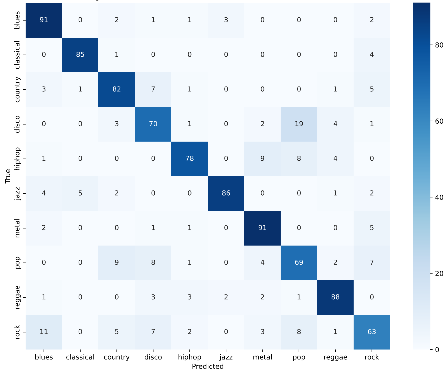
Stage 3 (CNN + Tabular Fusion) — Confusion Matrix (Test Set)
