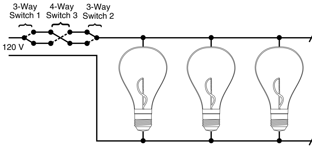
Figure 5-3 Four-Way Switch
