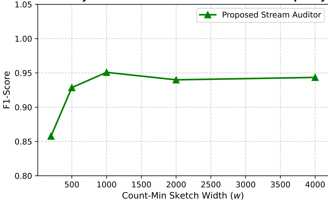
Accuracy Evaluation vs. Probabilistic Sketch Capacity
