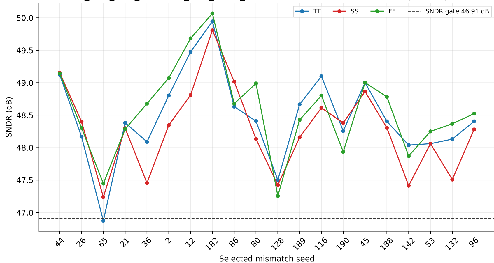
CMP_XM5_XM6_W8P2524_XM7_XM11_W16P8587 selected MC20: SNDR by analog PVT
