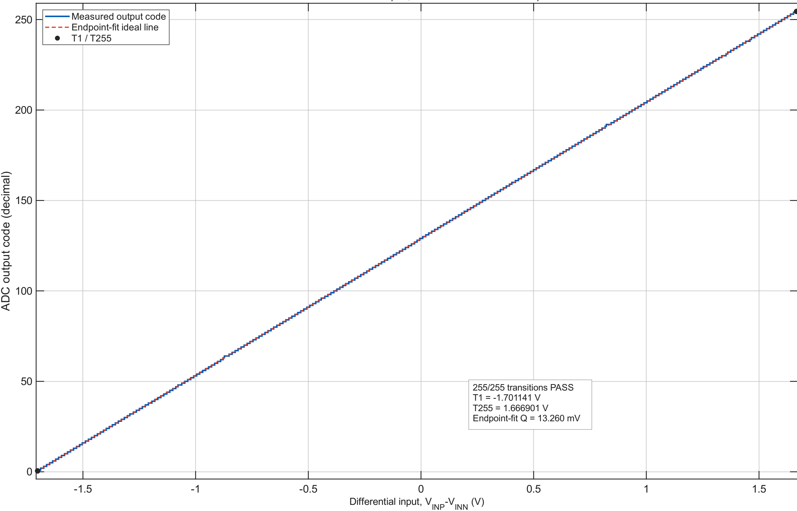
FULL STATIC Transfer Curve - Seed 44, TT XM5/XM6 W=8.2524 \mu\text{m} ; XM7/XM11 W=16.8587 \mu\text{m}
