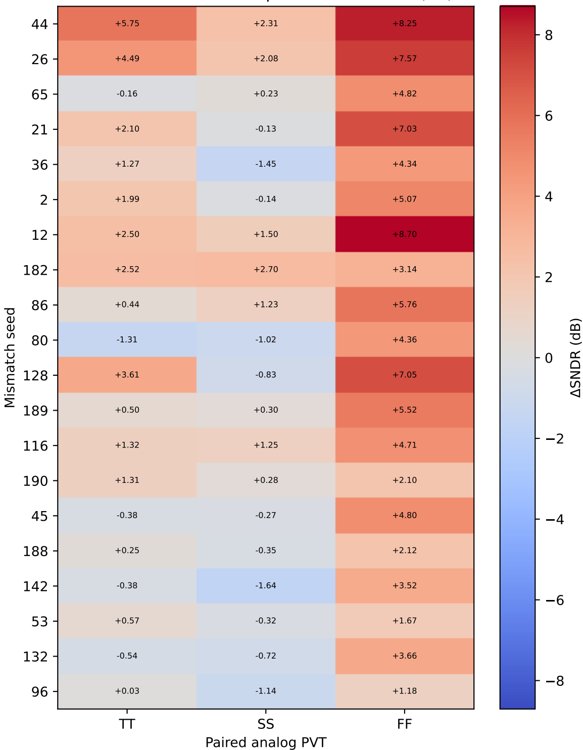
Resized minus T1P000 paired SNDR delta (dB)
