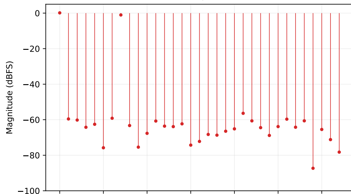
FF worst: seed 128, SNDR 47.26 dB
