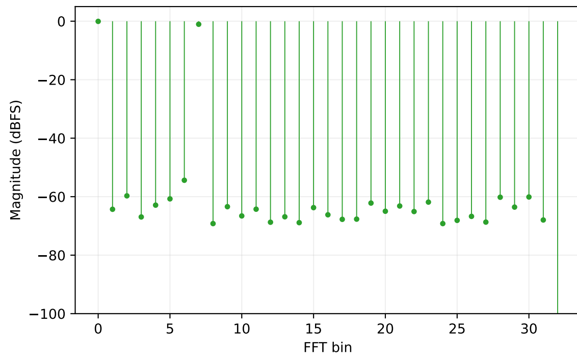
FF worst: seed 128, SNDR 47.26 dB
