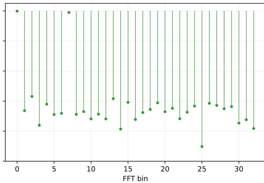
FF near-median: seed 86, SNDR 48.68 dB
