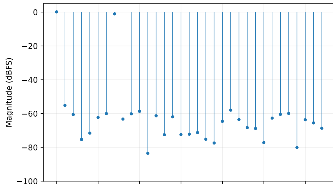
SS worst: seed 65, SNDR 47.24 dB
