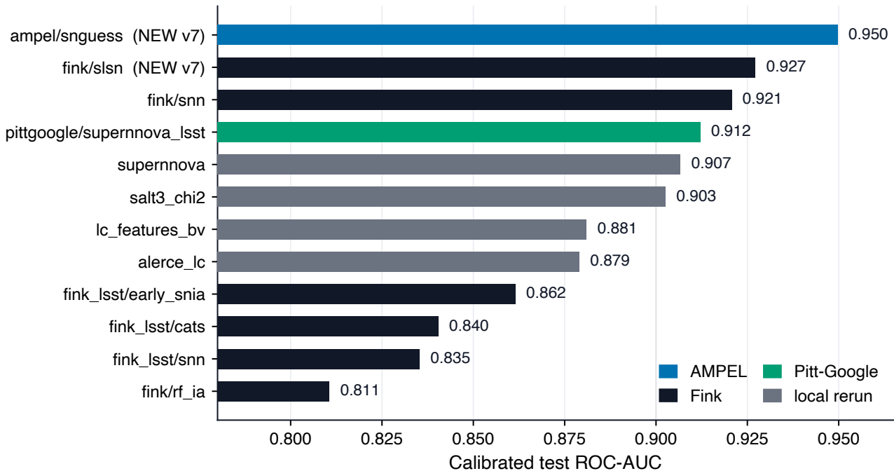
Twelve calibrated trust heads ranked by held-out AUC
