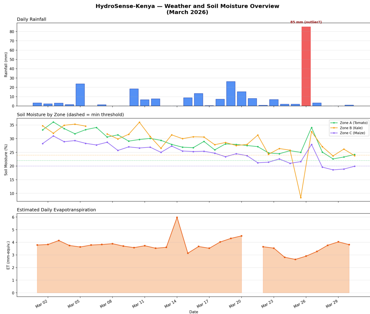
[Figure 1: level1_overview_plot.png — Weather and Soil Moisture Overview (March 2026)]
