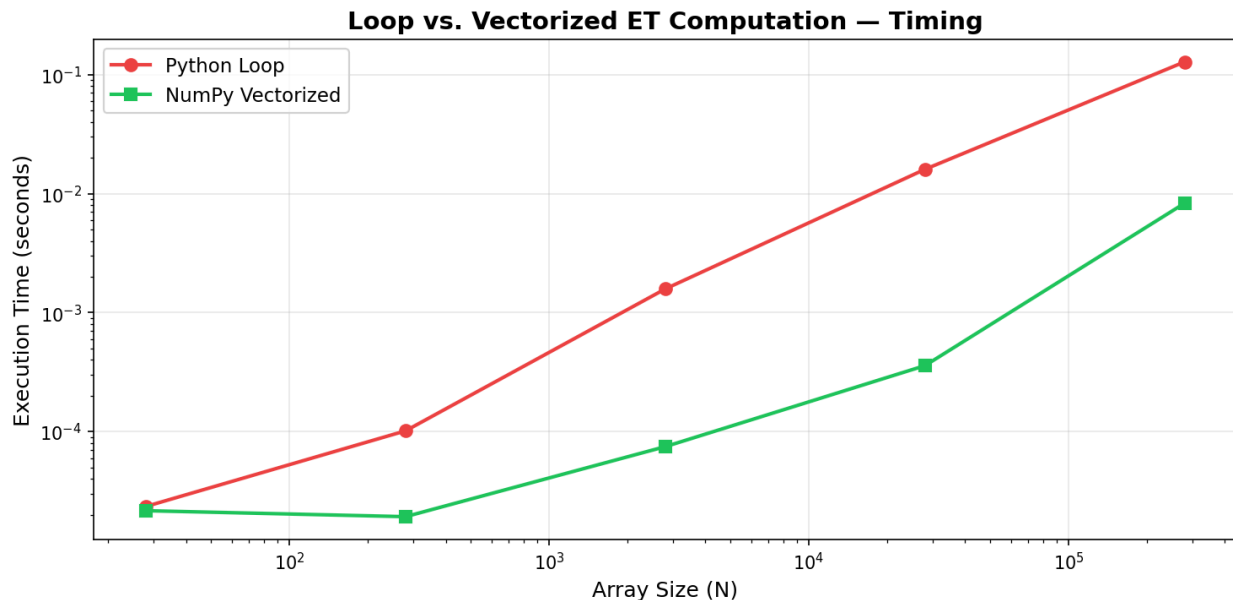
[Figure 2: level2_timing_comparison.png — Loop vs. Vectorized ET Computation Timing]
