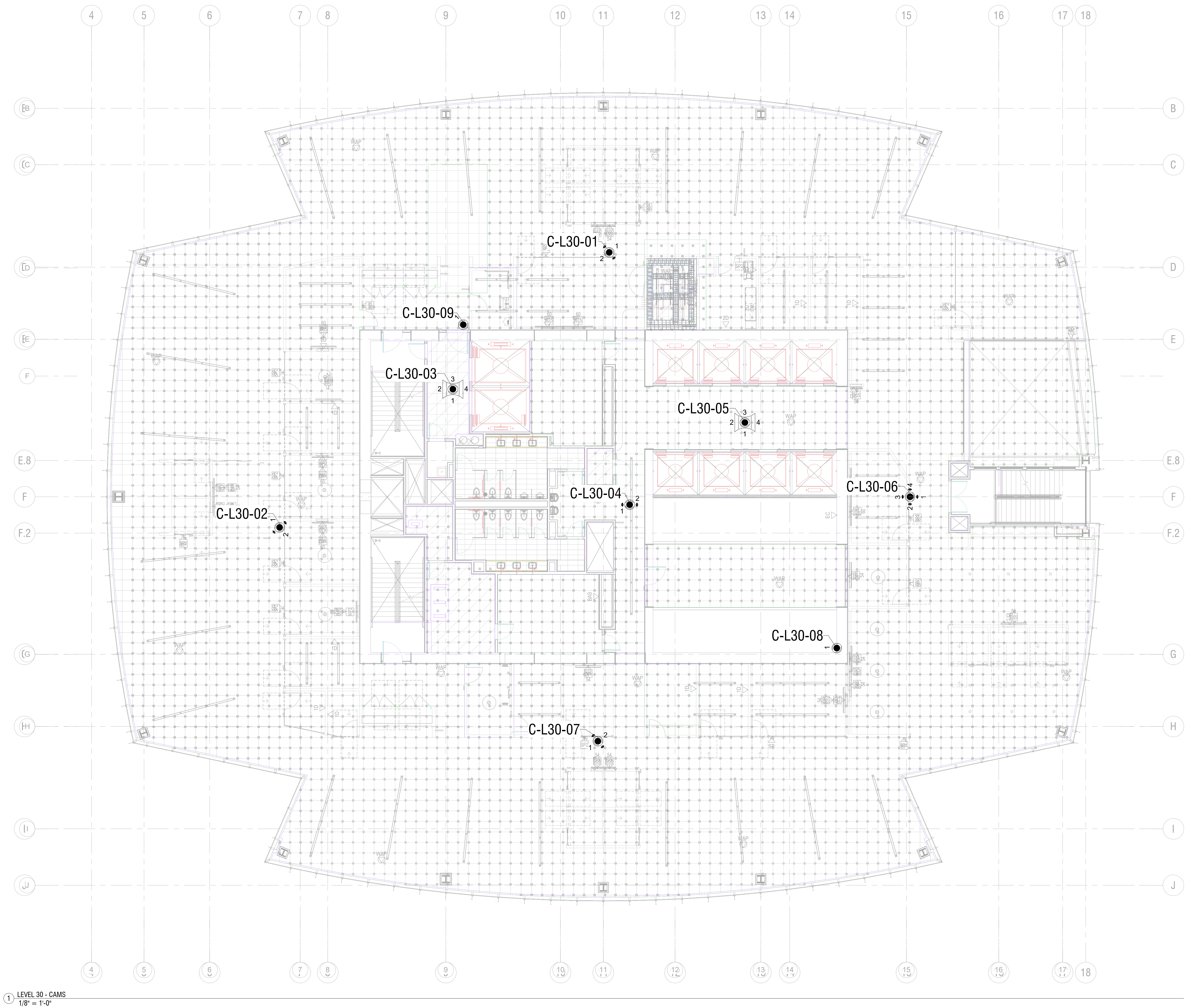
1 LEVEL 30 - CAMS 1/8" = 1'-0"
