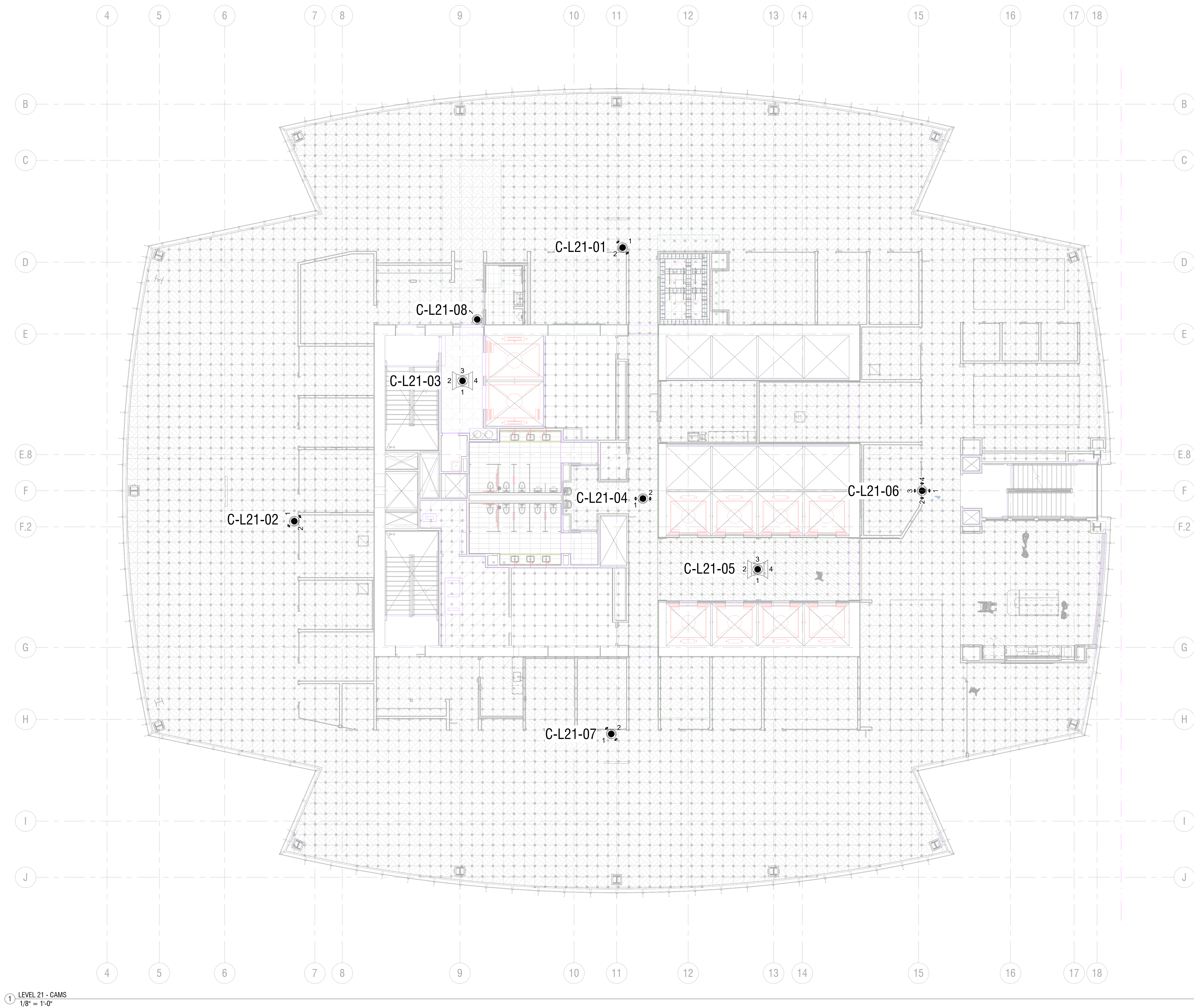
1 LEVEL 21 - CAMS 1/8" = 1'-0"
