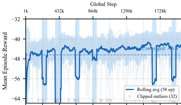
(a) Reward Convergence
