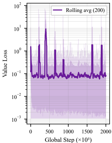
(b) Value Loss
