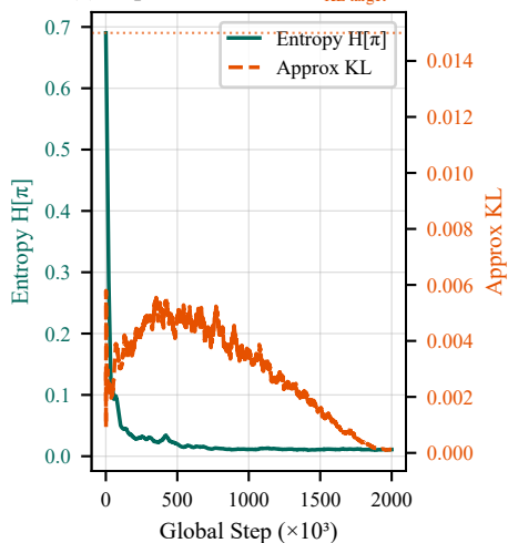
(c) Exploration &amp; KL Divergence
