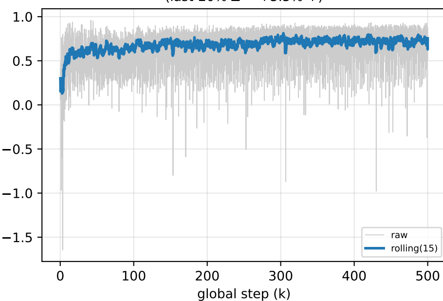
Critic explained var (last-20% \Delta = +5.5\% \uparrow )
