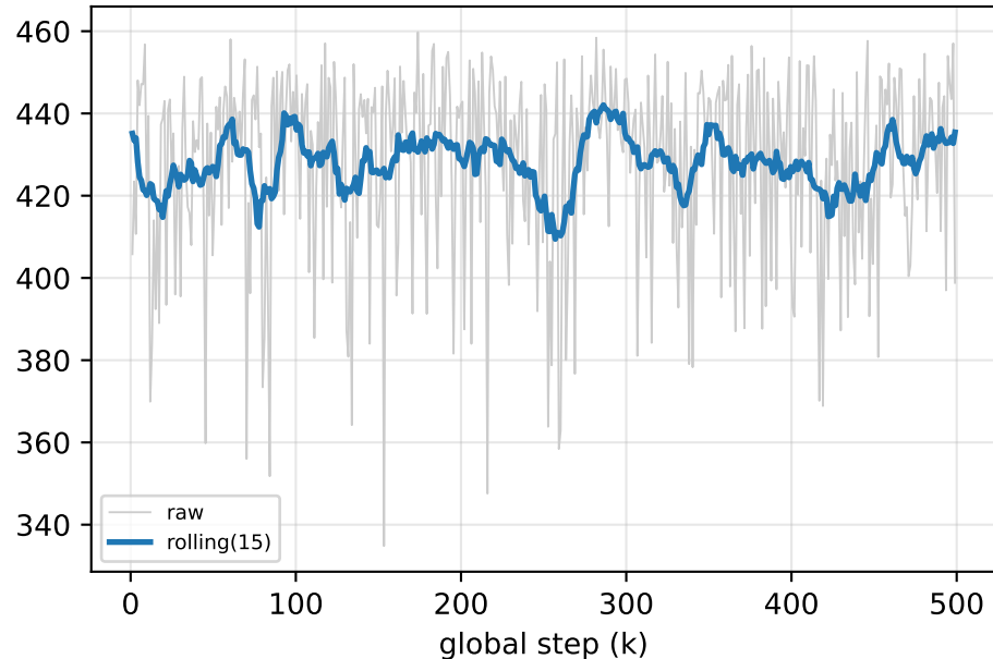
Throughput (veh/ep) (last-20% \Delta = -1.4\% \downarrow )
