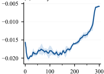
(c) Entropy
