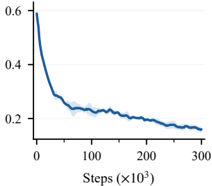
(c) Entropy
