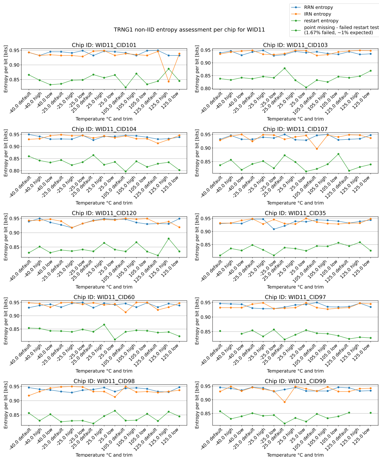
Figure 42: TRNG1 entropy assessment at all conditions for WID11.
