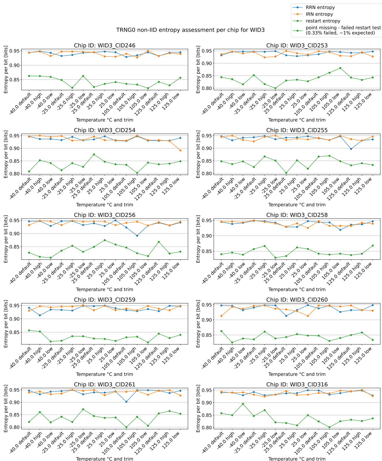
Figure 5: TRNG0 entropy assessment at all conditions for WID3.
