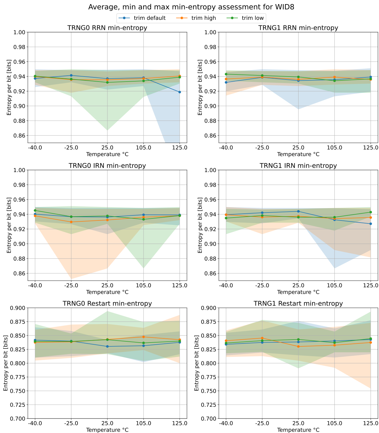
Figure 37: Combined entropy assessment for WID8.
