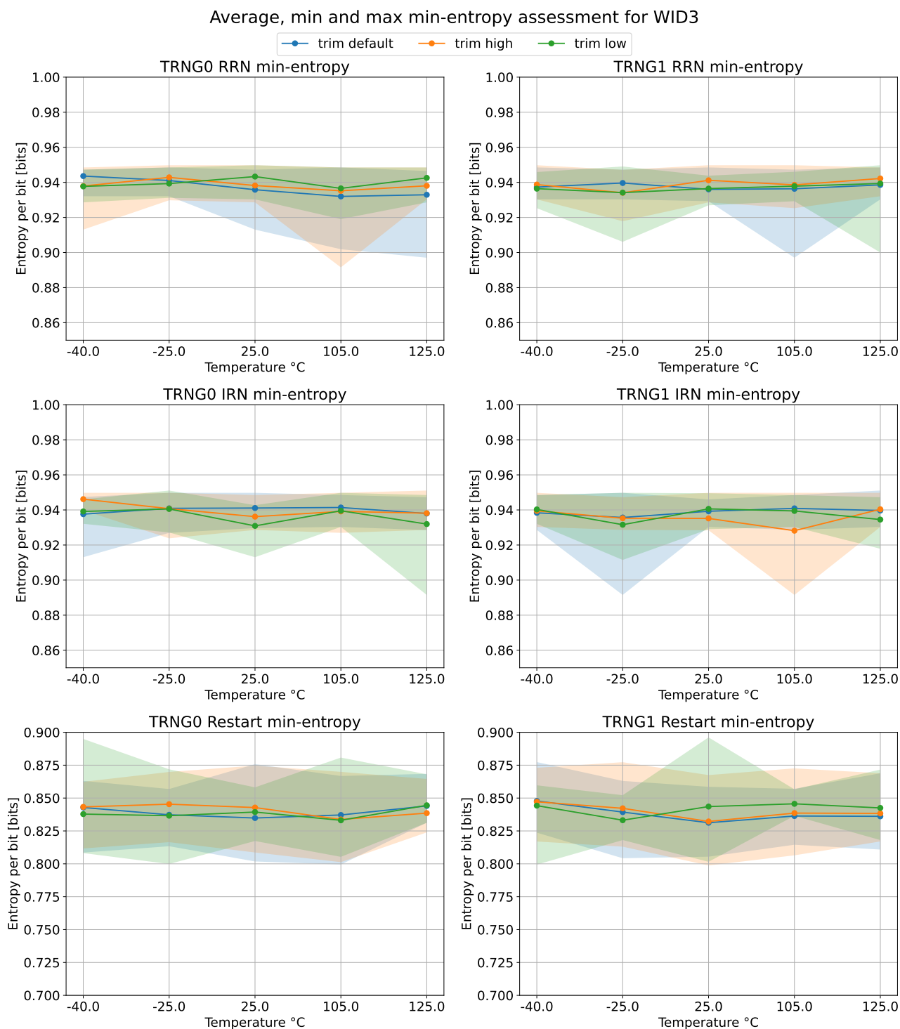
Figure 4: Combined entropy assessment for WID3.
