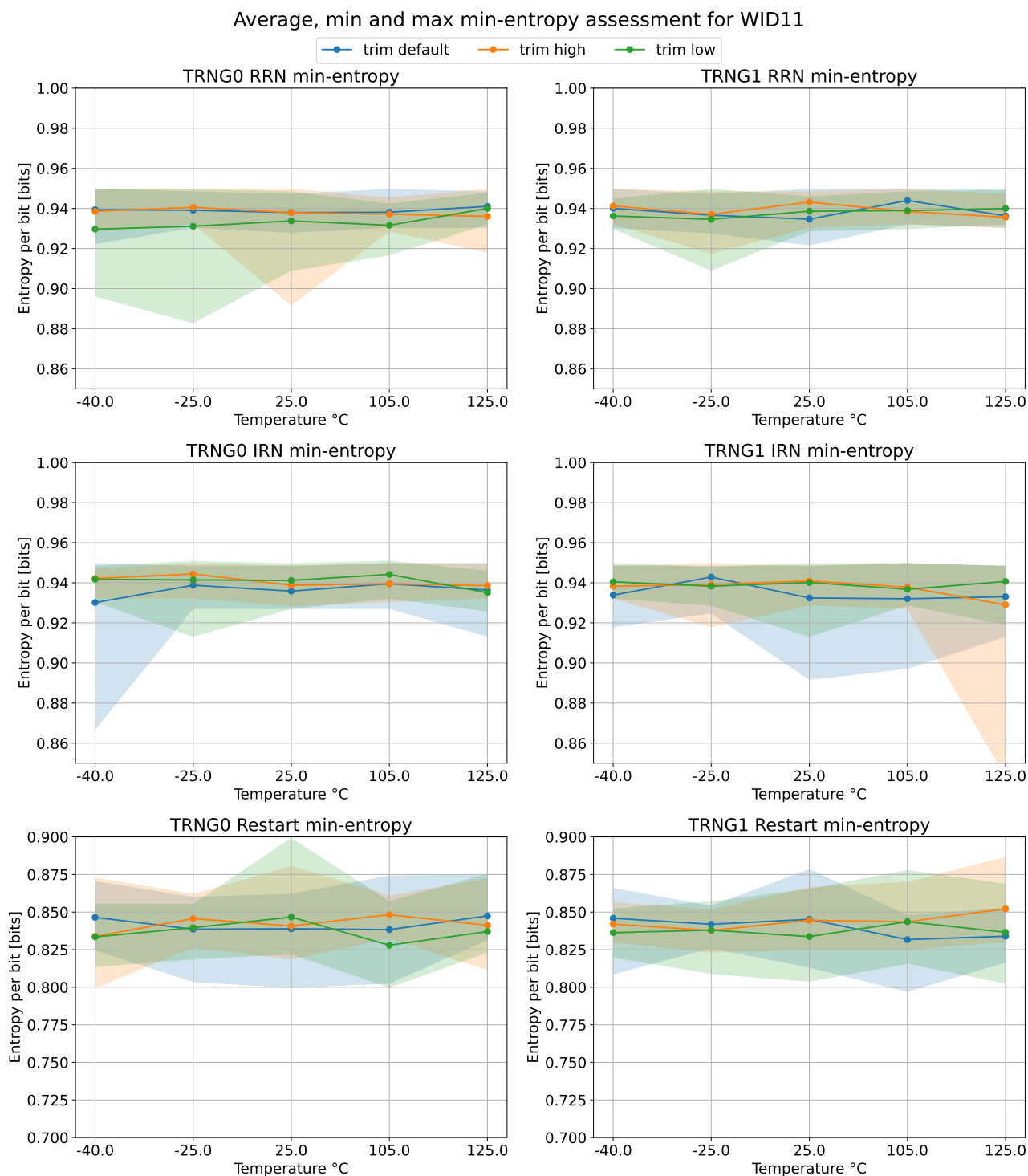
Figure 38: Combined entropy assessment for WID11.
