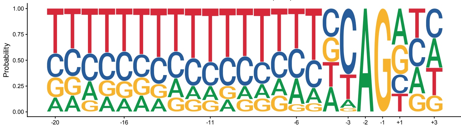
annotated 3'SS (5,000 sampled) (n=5000)
