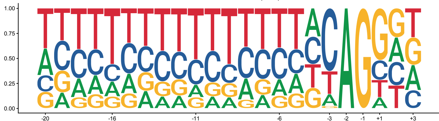
WT-associated novel A3SS (n=108)
