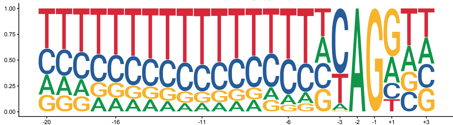
annotated 3'SS (5,000 sampled) (n=5000)
