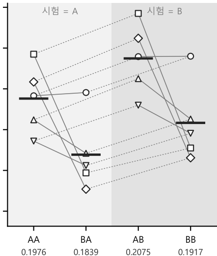
CPTransformer
