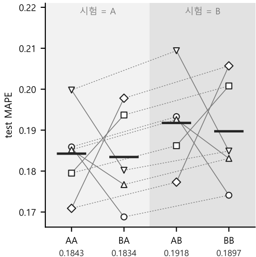
CPMLP
