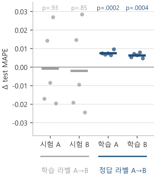
CPMLP
