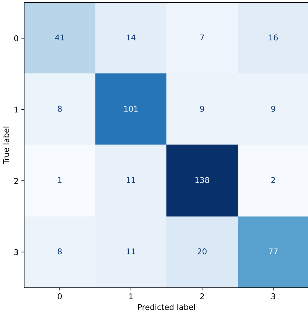
CQT Confusion Matrix
