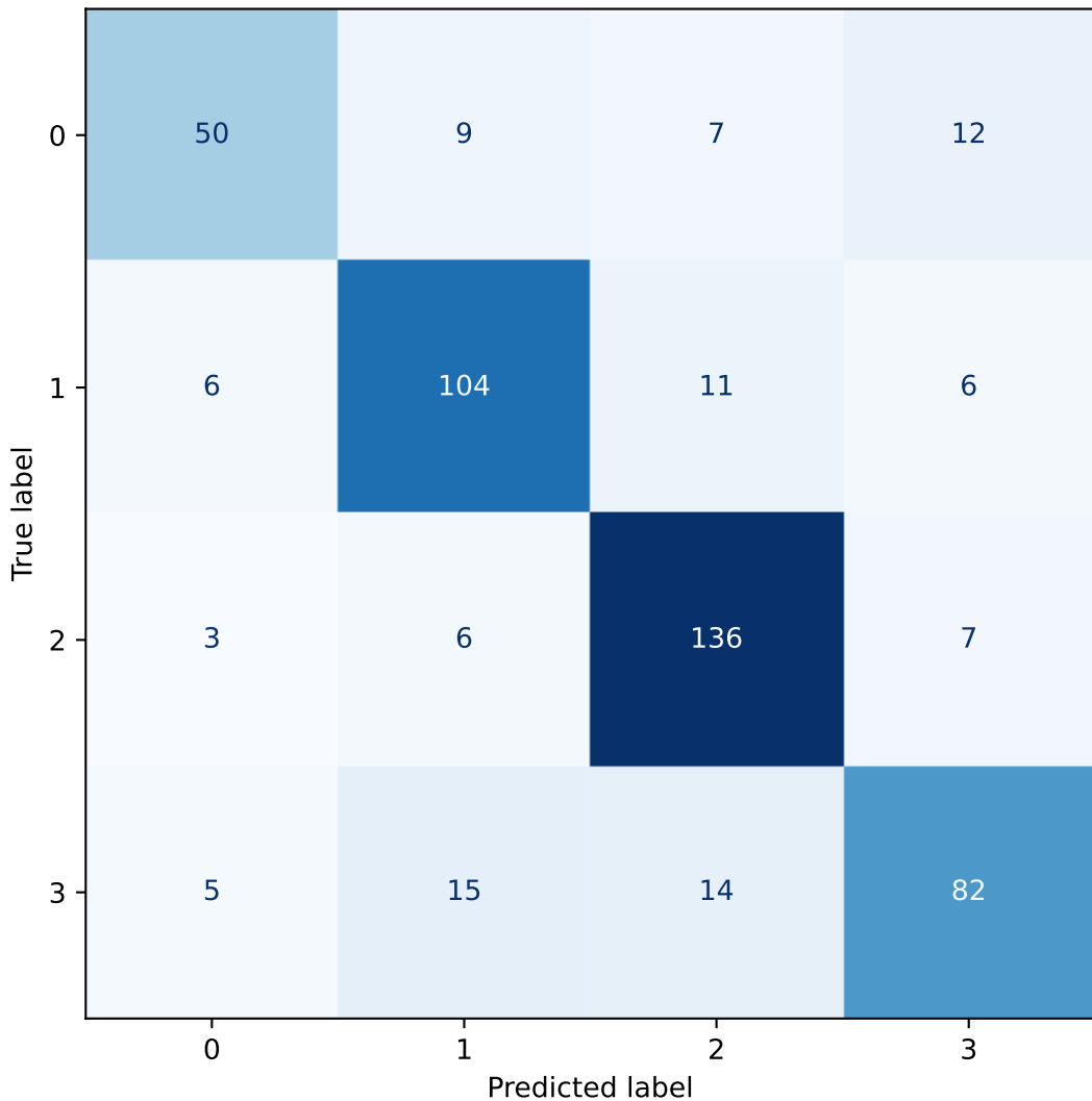
MFCC Confusion Matrix
